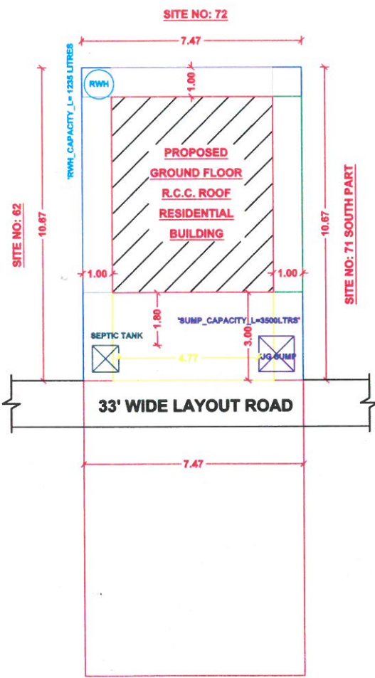
SITE PLAN
