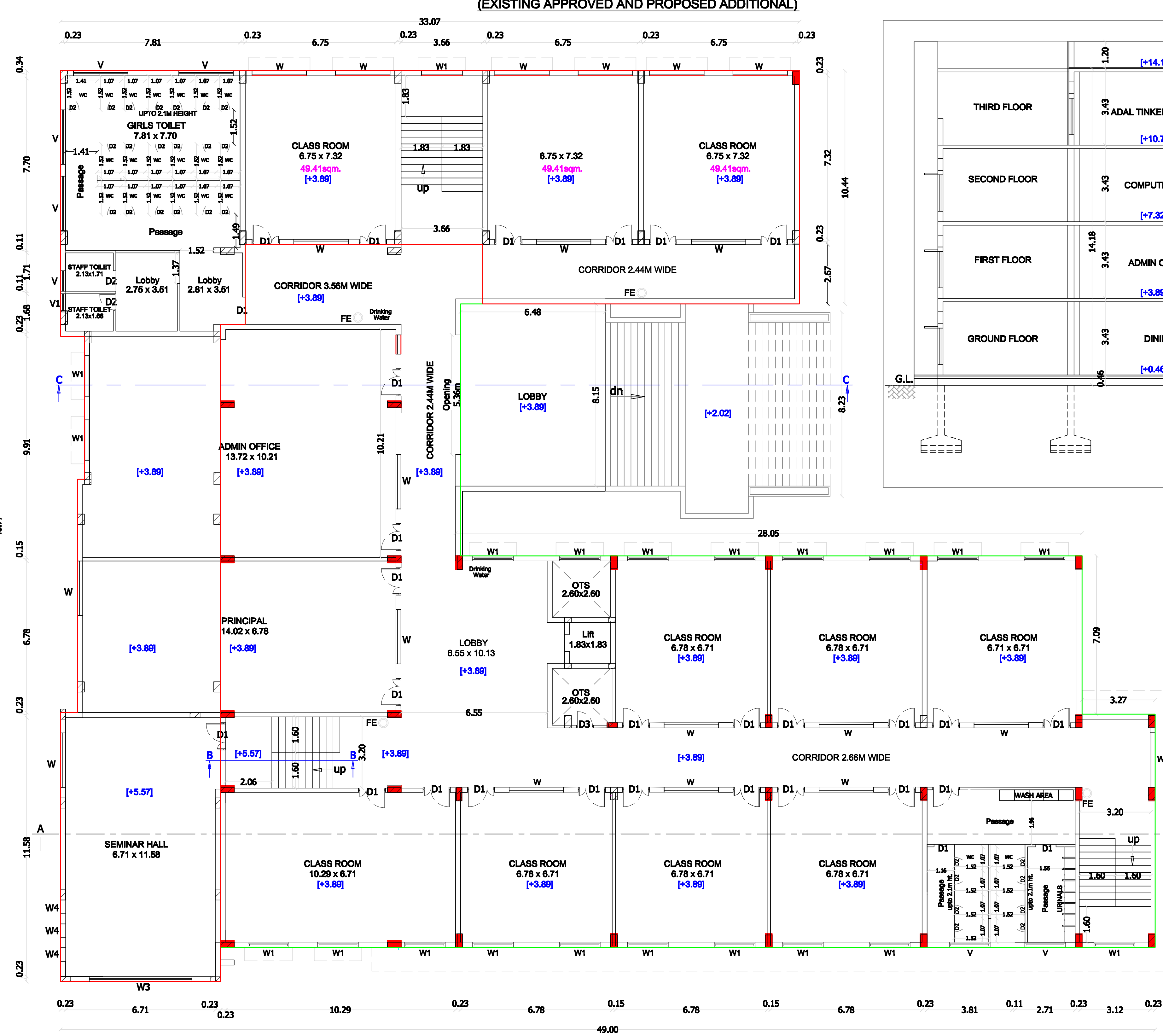
FIRST FLOOR PLAN (EXISTING APPROVED AND PROPOSED ADDITIONAL)
