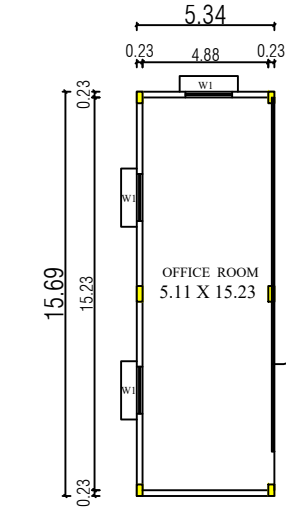
OFFICE FLOOR PLAN
