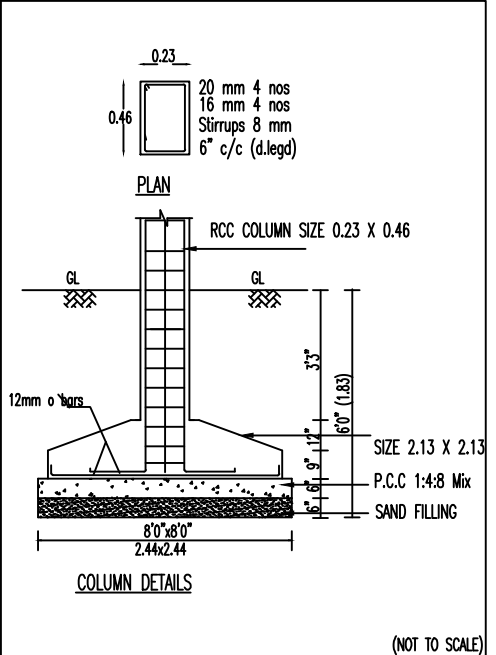
COLUMN DETAILS
