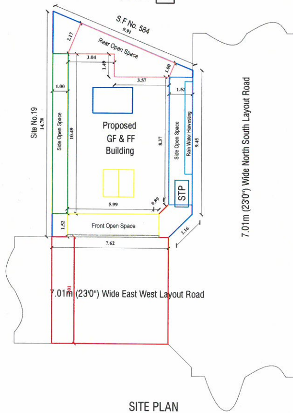
SITE PLAN
