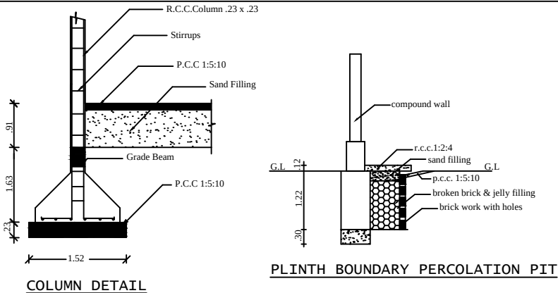
COLUMN DETAIL
