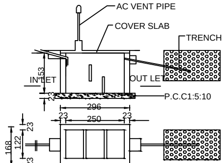
SEPTIC TANK
