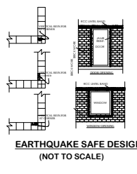
SEISMIC REINFORCEMENT DETAILS
