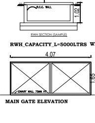
RAIN WATER HARVESTING DETAIL
