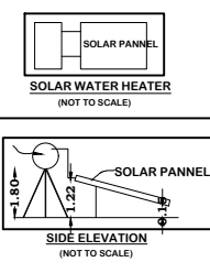
FOUNDATION DETAILS
