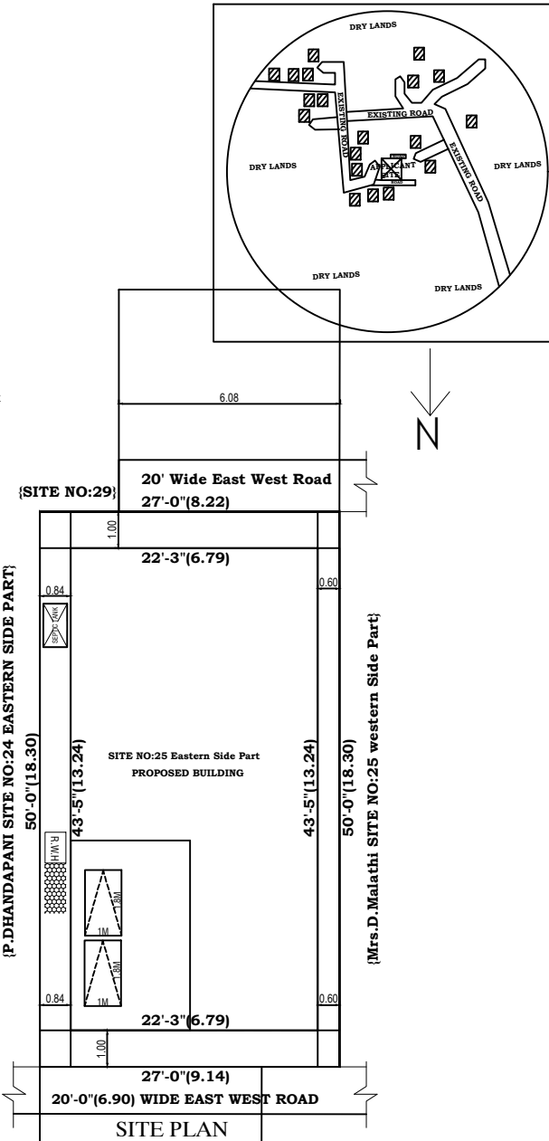
SITE PLAN
