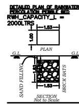
DETAILED PLAN OF RAINWATER DISPOSAL SYSTEM WITH RUN CAPACITY L = 2000LTRS
