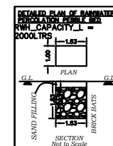
DETAILED PLAN OF RAINWATER DISPOSAL SYSTEM WITH RUN CAPACITY L = 2000LTRS
