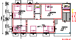
PROPOSED GROUND FLOOR PLAN
