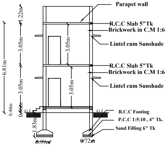
SECTION-AB
