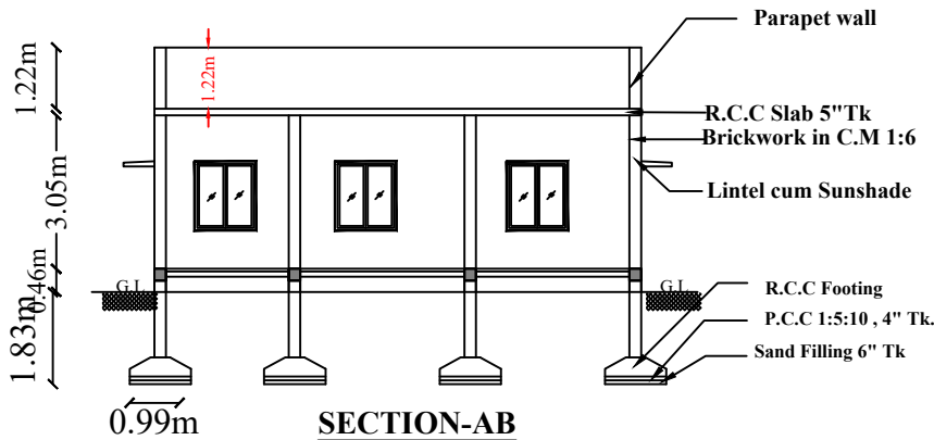
SECTION-AB
