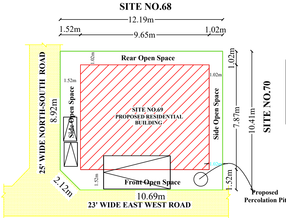
SITE PLAN
