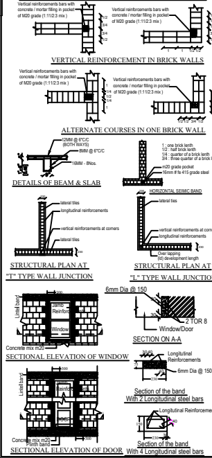
EARTHQUAKE SAFE DESIGN DETAILS:
