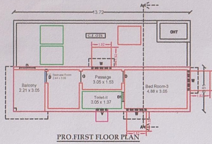
PRO. FIRST FLOOR PLAN
