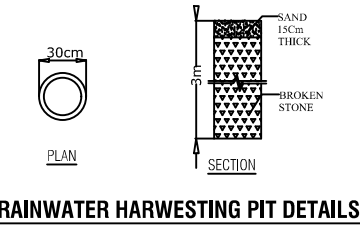
RAINWATER HARVESTING PIT DETAILS
