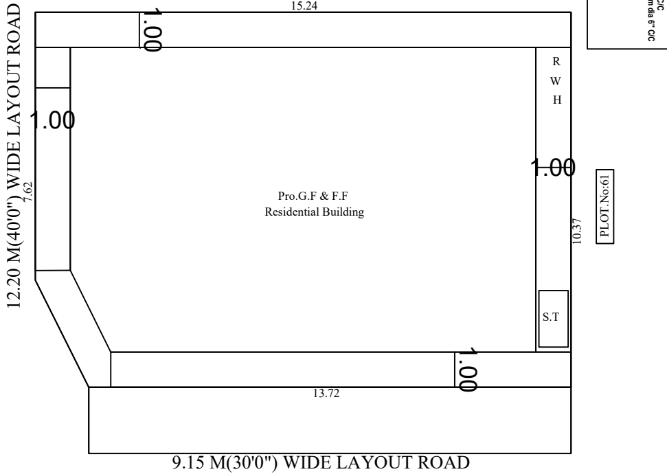
SITE PLAN
