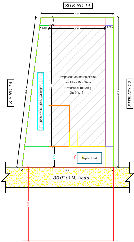
Site Plan
