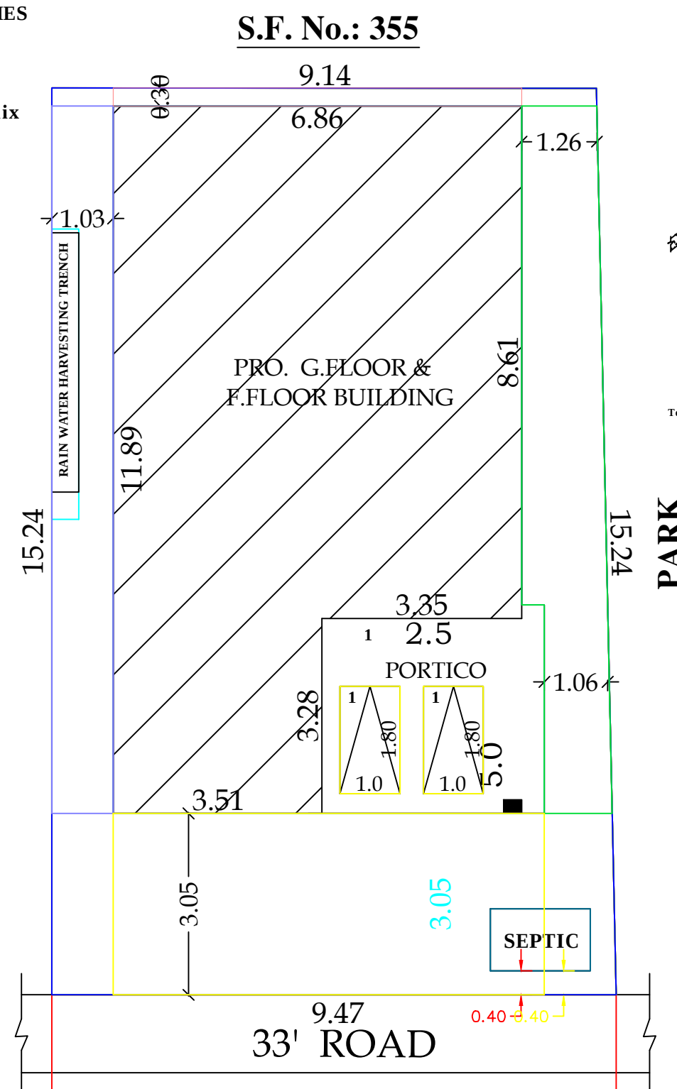
SITE PLAN
