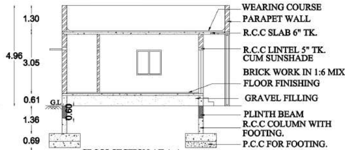
CROSS SECTION AT A-A
