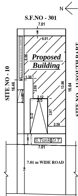
SITE PLAN
