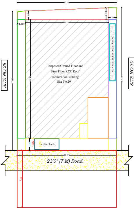
Site Plan
