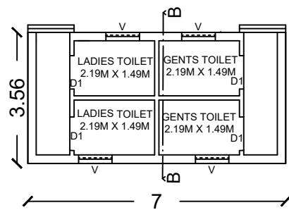
TOILET BLOCK
