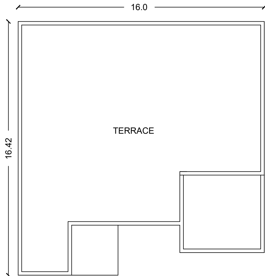
TERRACE FLOOR
