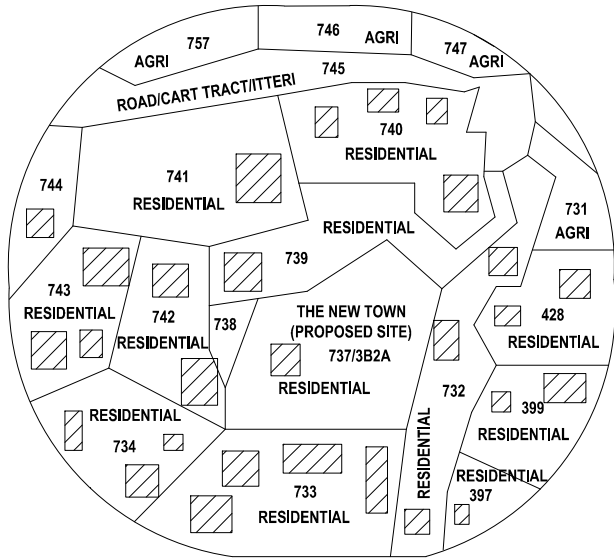
TOPO PLAN
