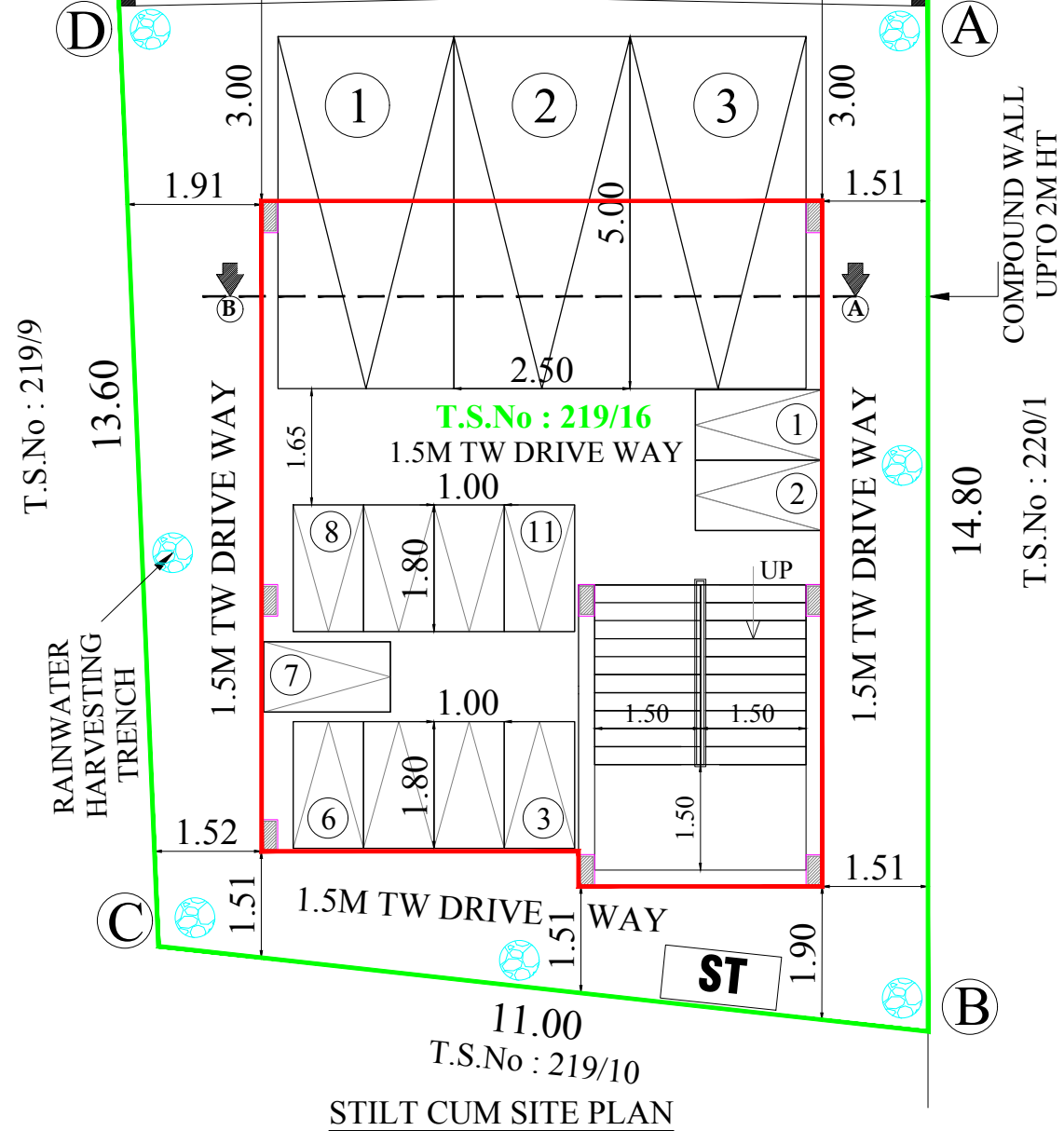
STILT CUM SITE PLAN
