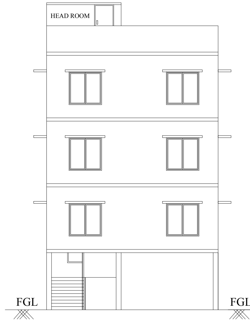
FRONT ELEVATION
