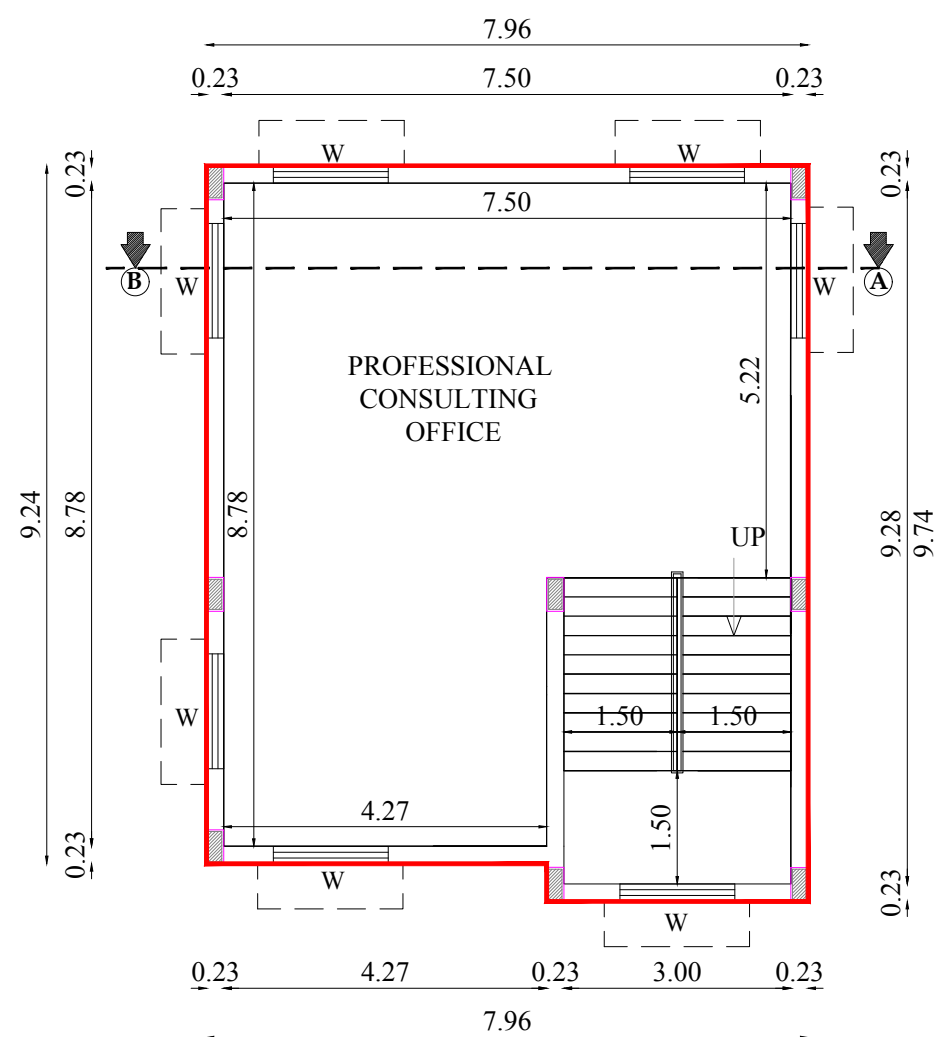
TYPICAL FLOOR PLAN (FIRST & SECOND FLOORS)
