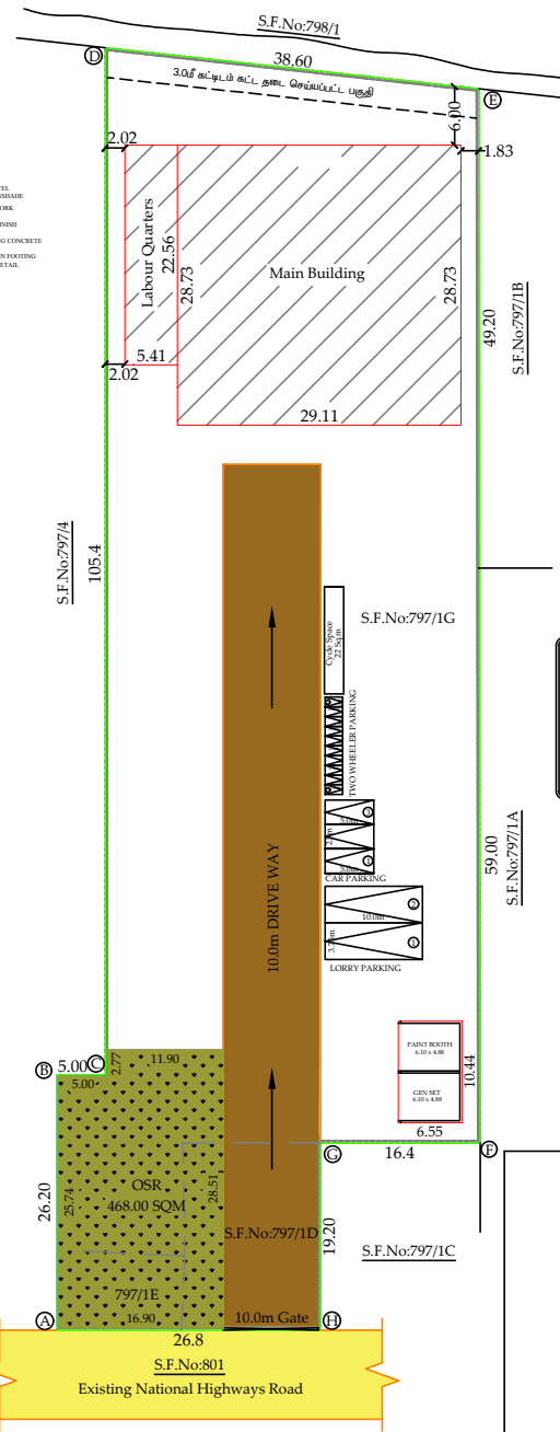
SITE PLAN
