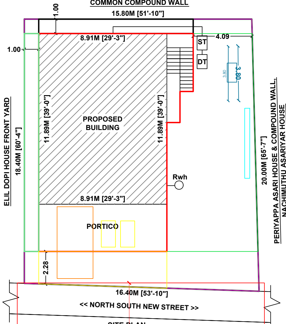
SITE PLAN
