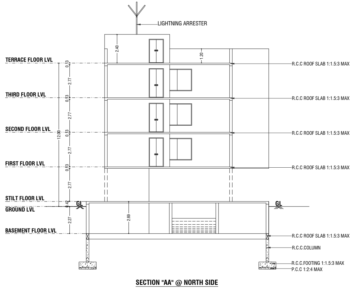
SECTION "AA" @ NORTH SIDE
