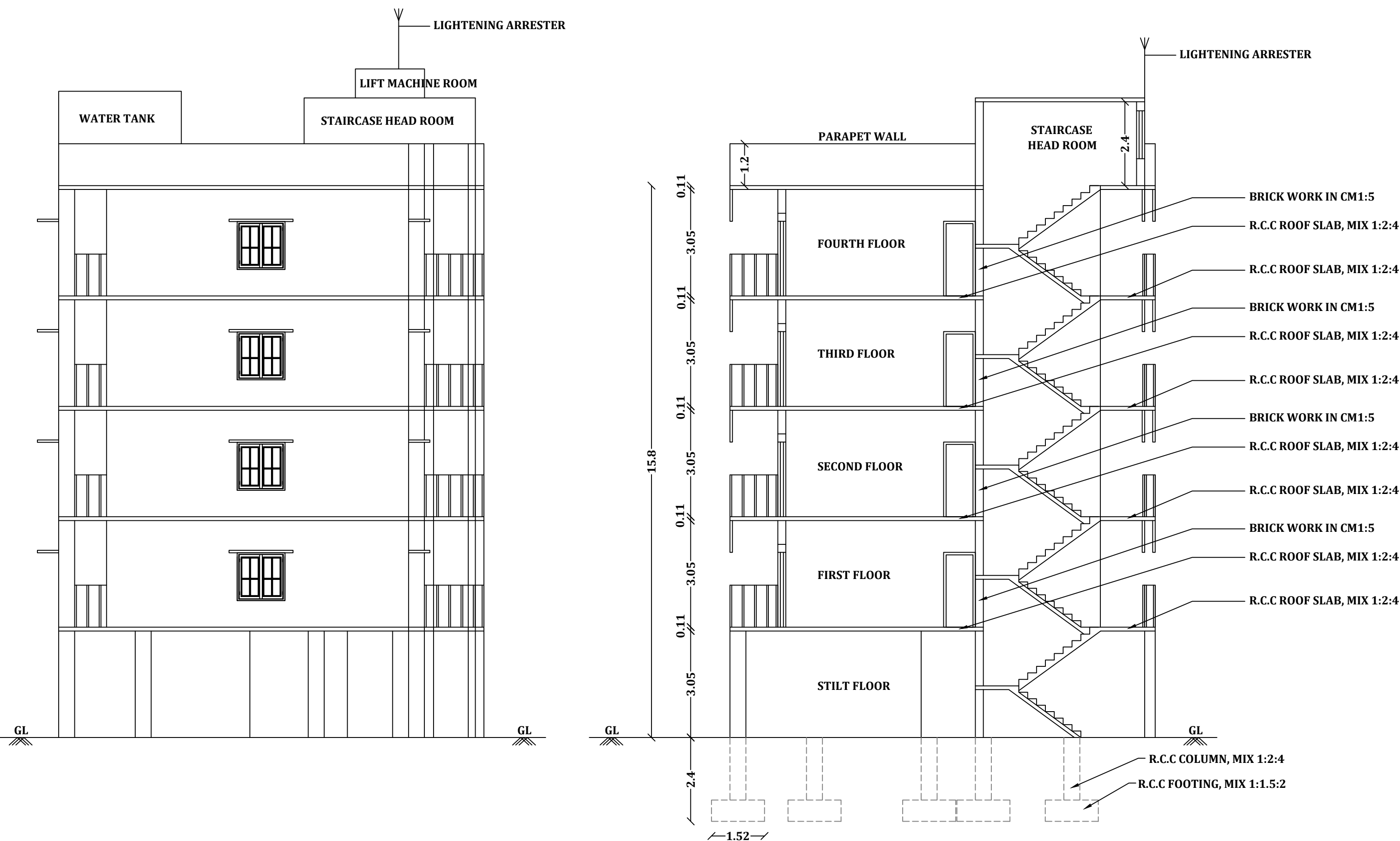
FRONT ELEVATION
