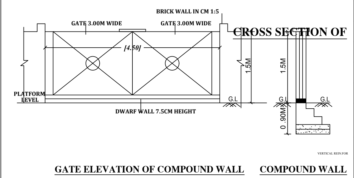
GATE ELEVATION OF COMPOUND WALL
