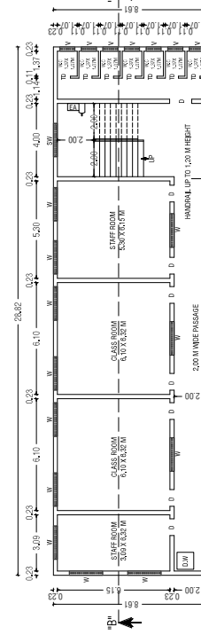
TYPICAL (FIRST & SECOND) FLOOR PLAN
