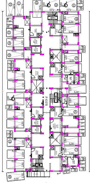
TYPICAL FLOOR PLAN-1
