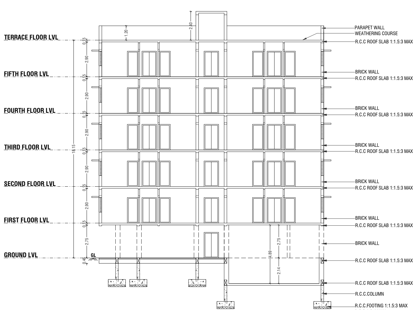
SECTION PLAN @ NORTH SIDE
