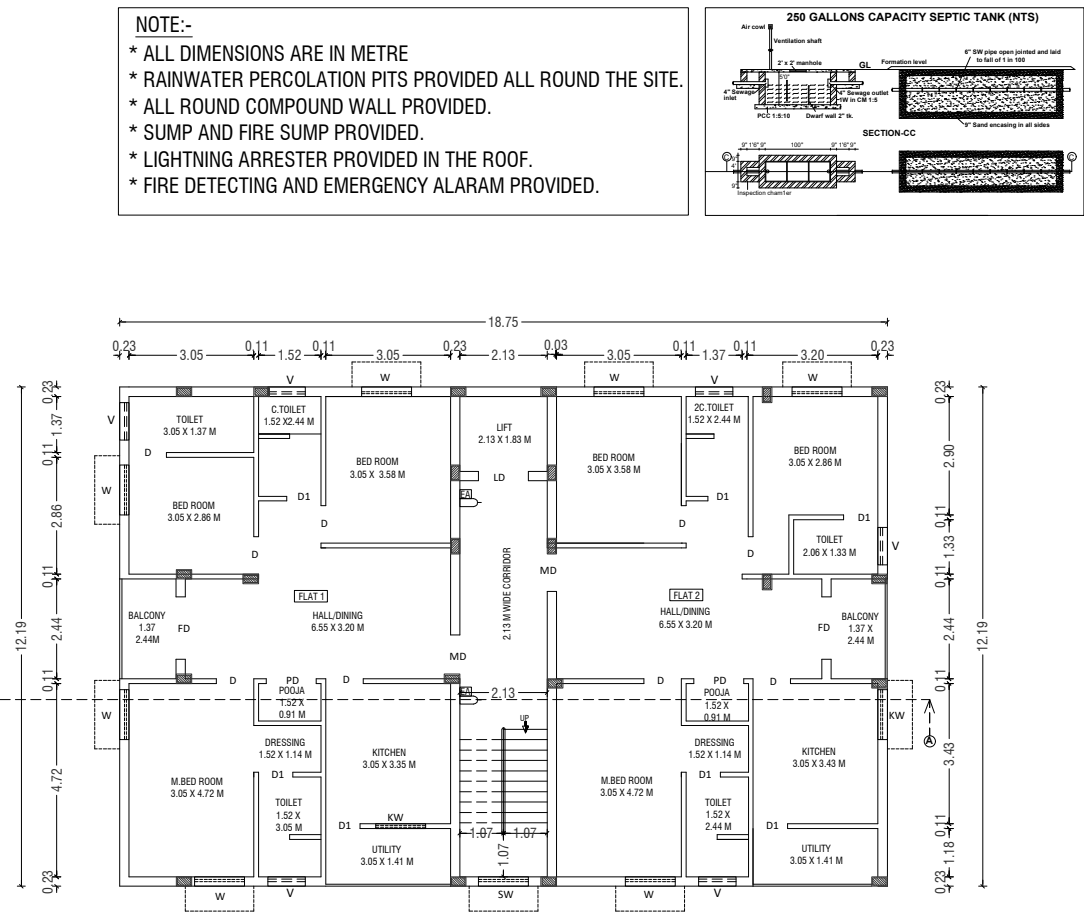
TYPICAL (FIRST, SECOND, THIRD, FOURTH & FIFTH) FLOORS PLAN
