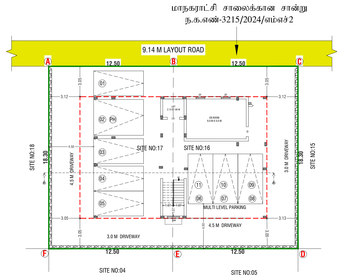
SITE CUM STILT FLOOR PLAN
