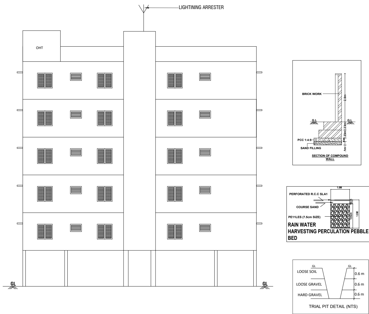
ELEVATION @ NORTH SIDE
