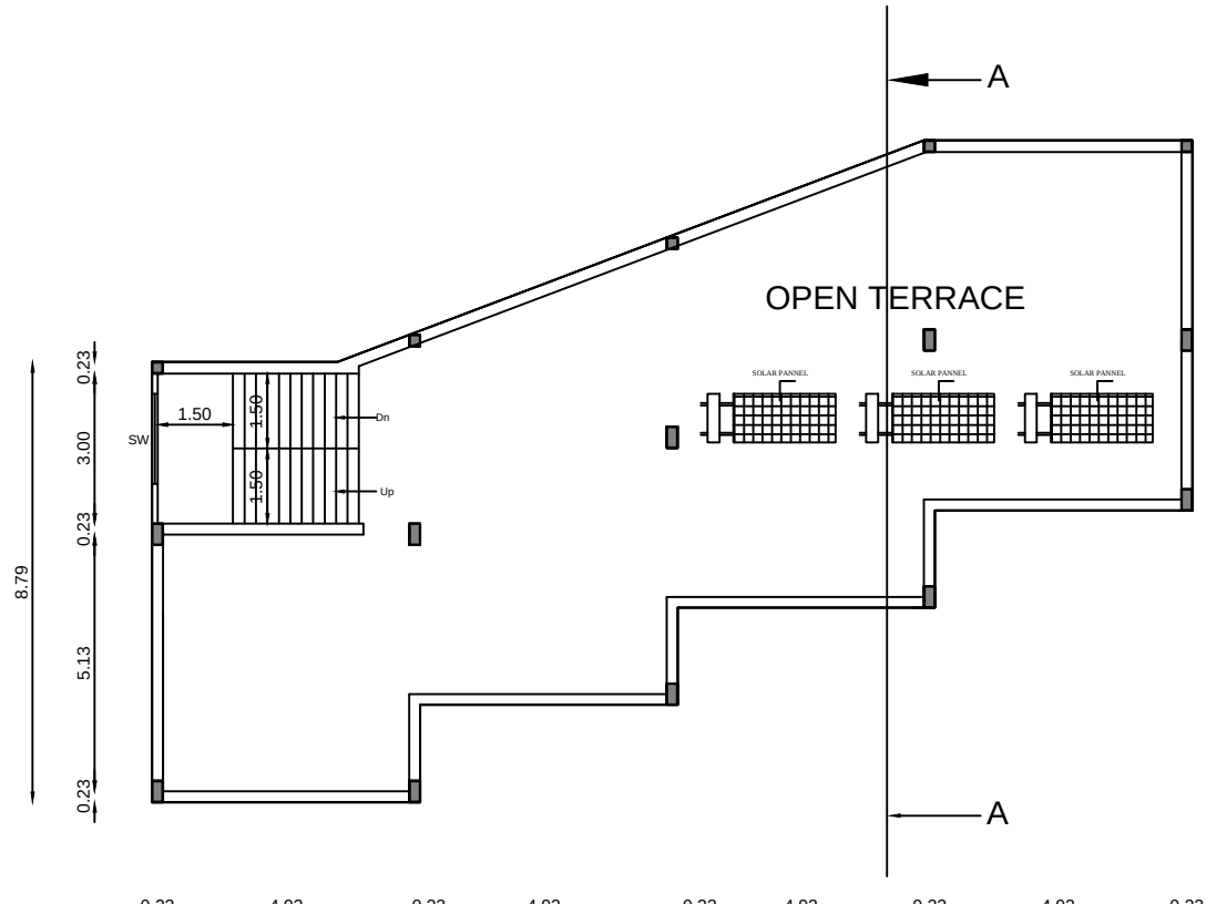
TERRACE FLOOR PLAN BLOCK NO :2
