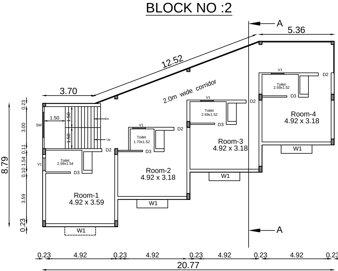
FIRST FLOOR PLAN BLOCK NO :2
