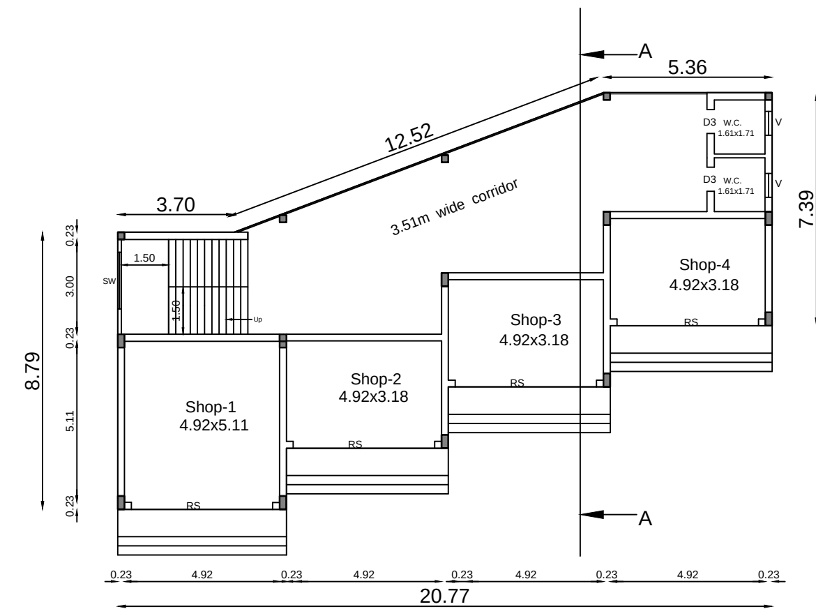
GROUND FLOOR PLAN BLOCK NO :2
