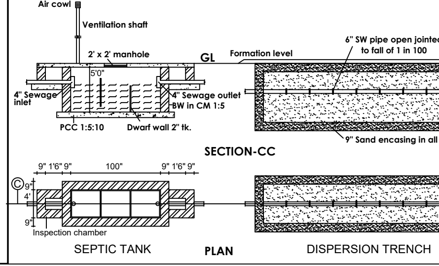
1000 GALLONS CAPACITY SEPTIC TANK (NTS)
