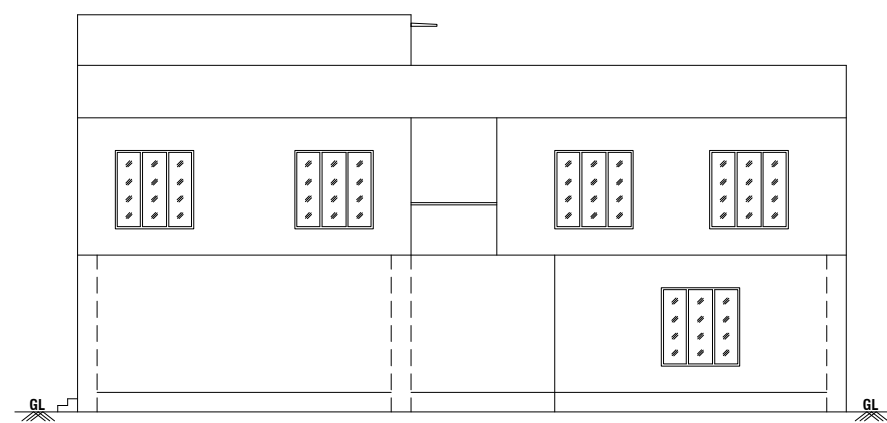
ELEVATION @ EAST SIDE
