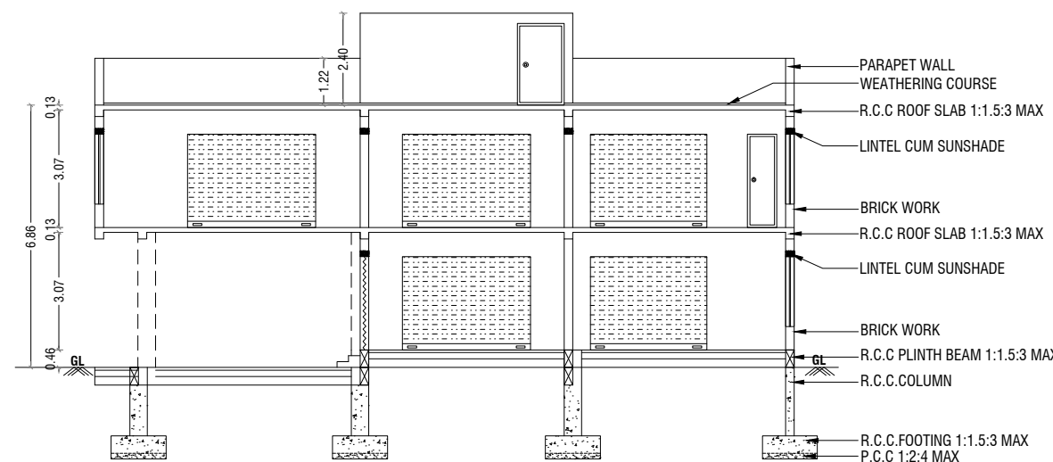
SECTION @ SOUTH SIDE
