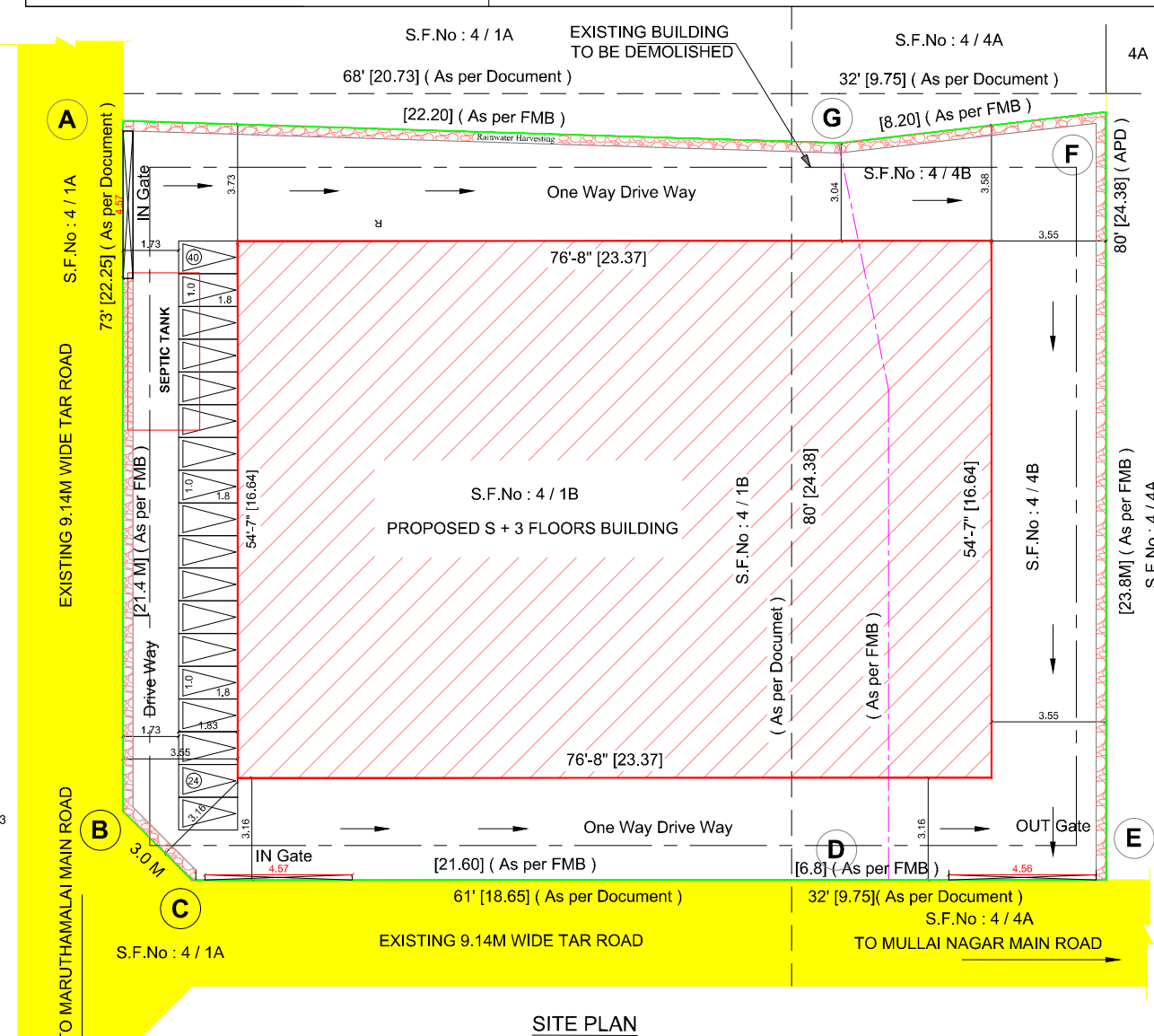
SITE PLAN
