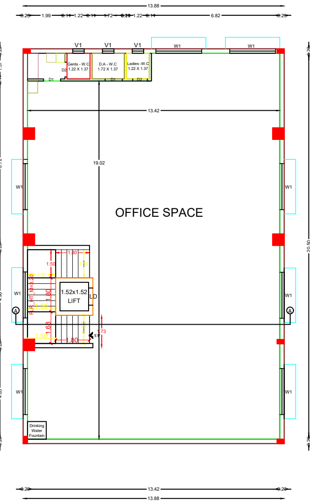
TYPICAL_FLOOR_PLAN=2,3 (SECOND AND THIRD FLOOR PLAN)
