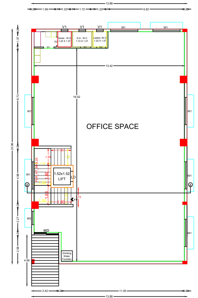
TYPICAL_FLOOR_PLAN=1 (FIRST FLOOR PLAN)
