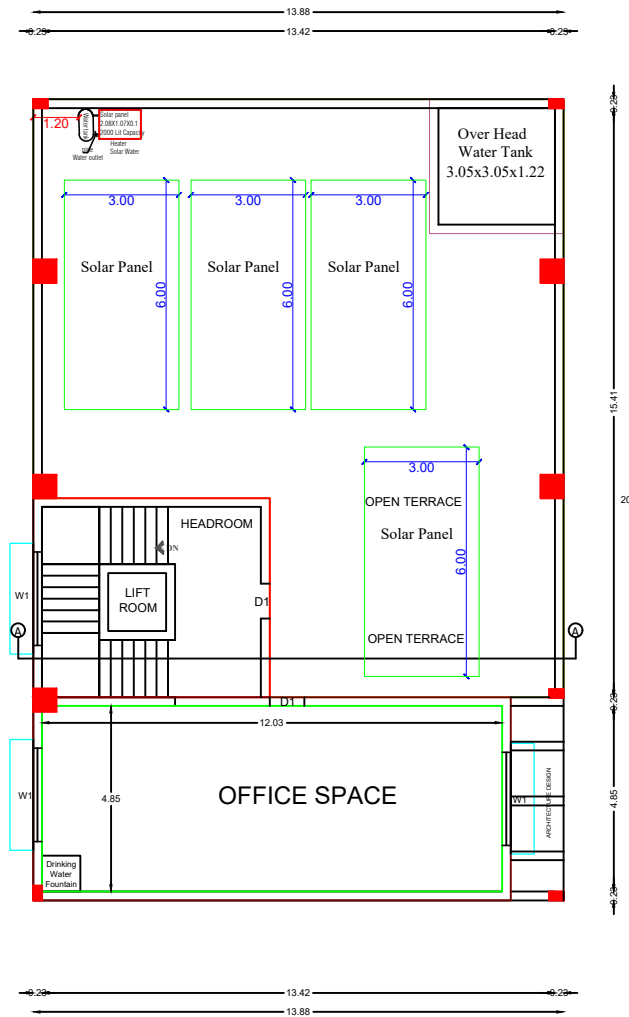
TYPICAL_FLOOR_PLAN=4 (FOURTH FLOOR PLAN)
