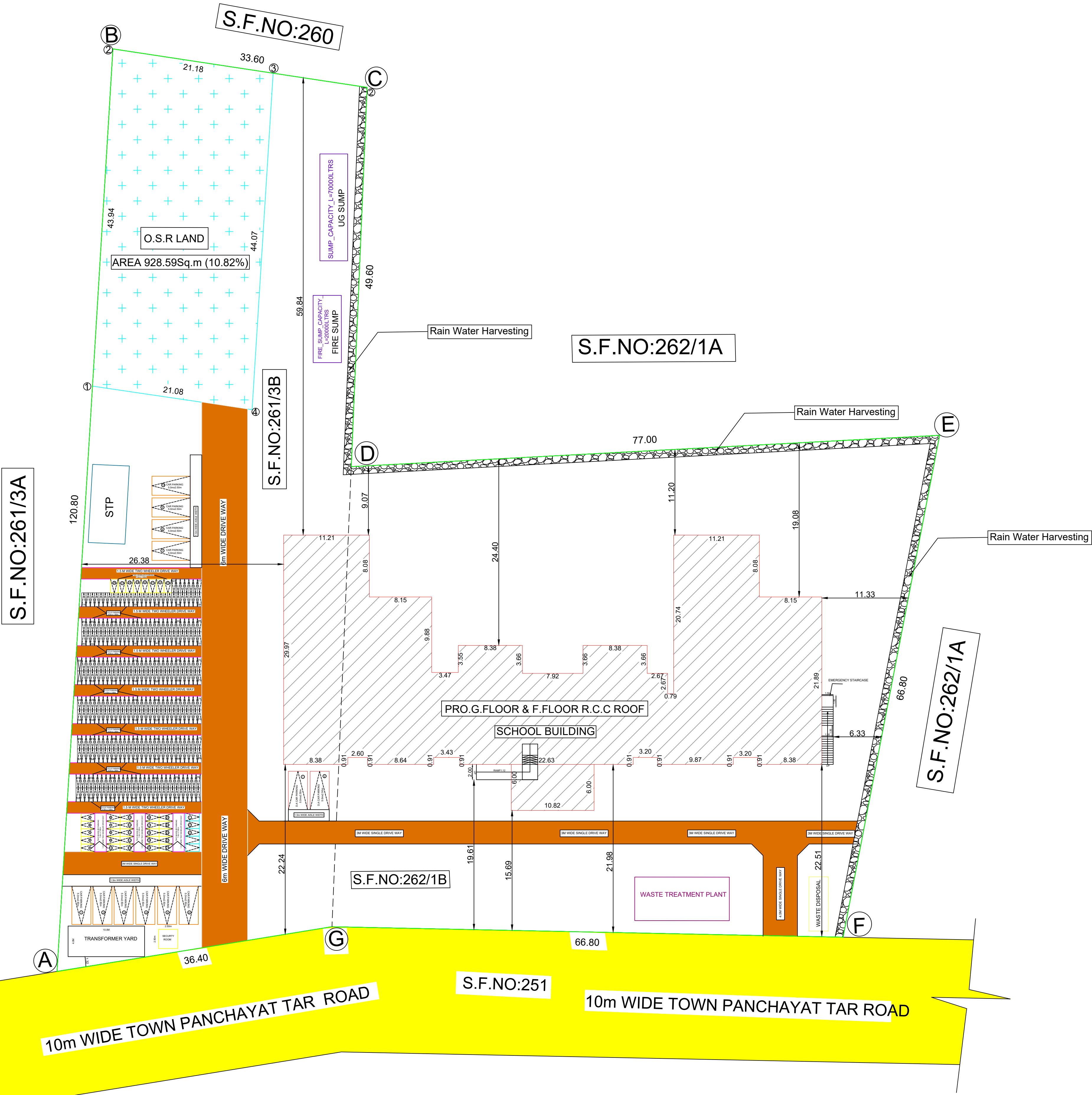
SITE PLAN
