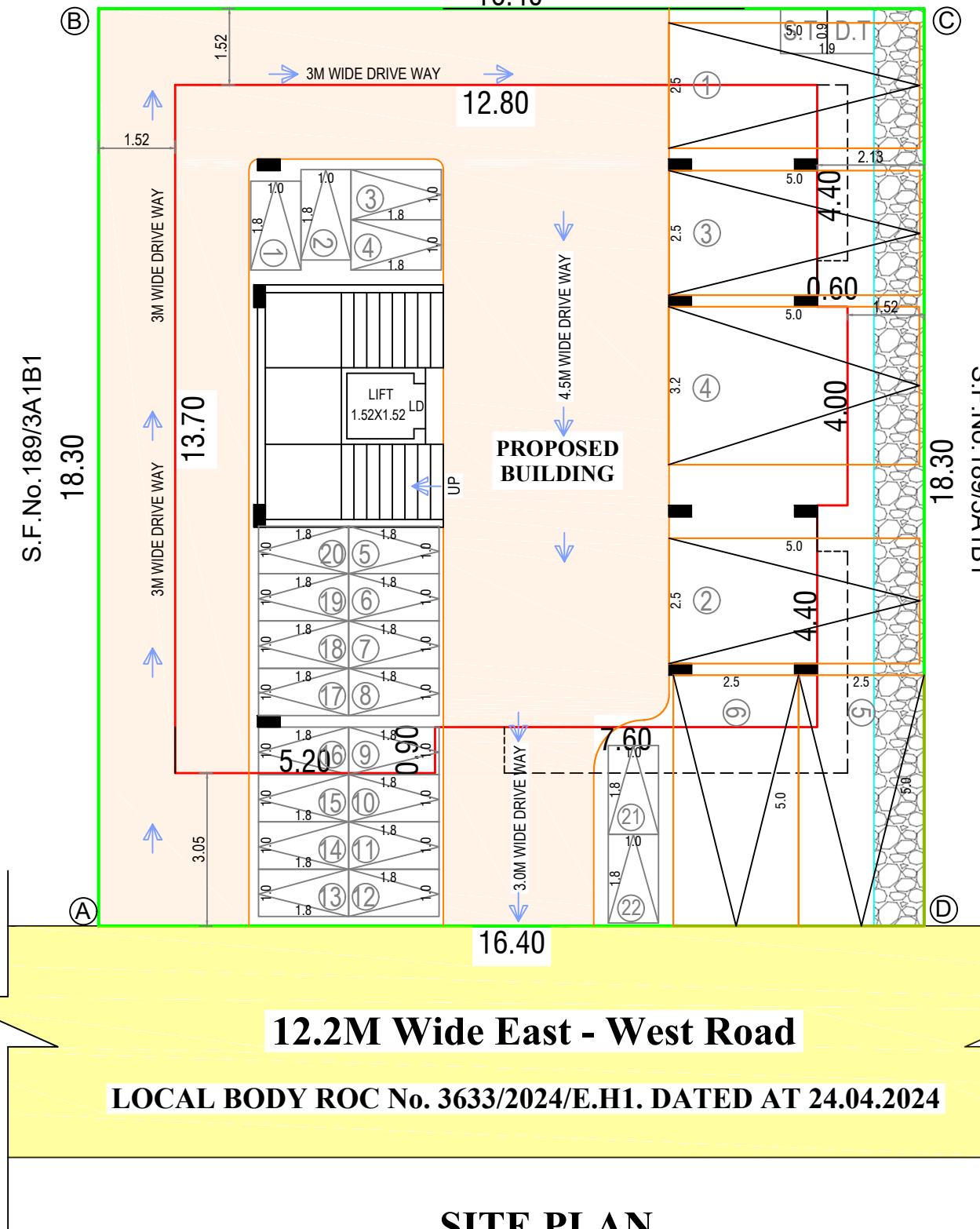
SITE PLAN
