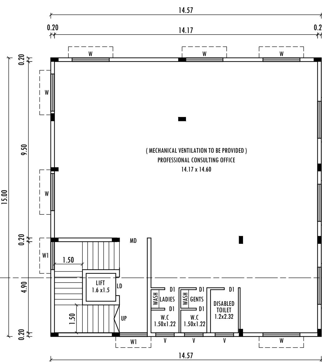
FIRST & SECOND FLOOR PLAN
