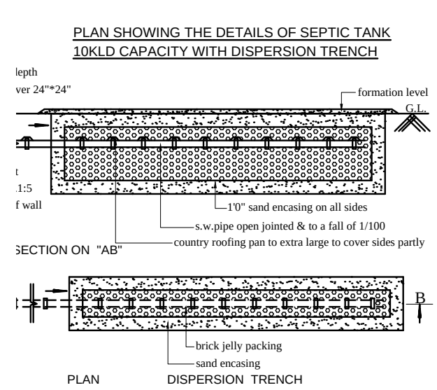
SEPTIC TANK
