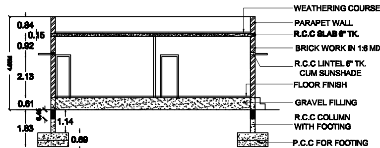
CROSS SECTION AT A-A
