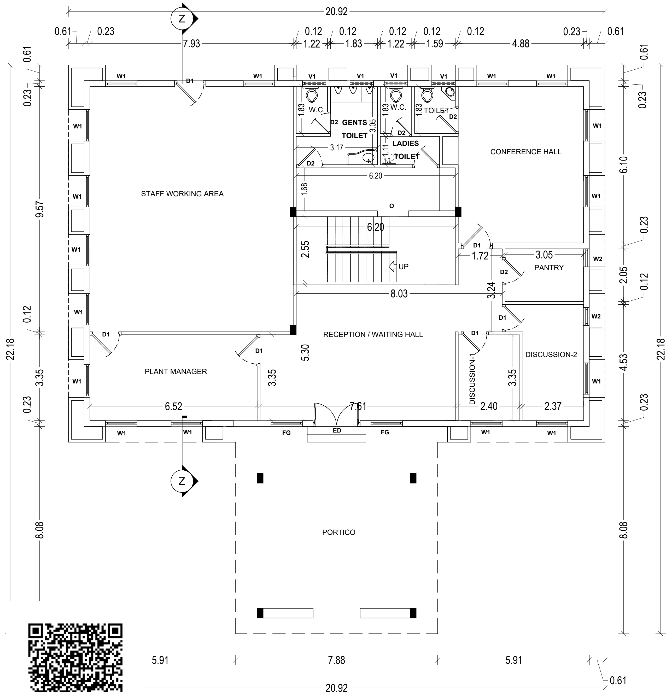
GROUND FLOOR PLAN ADMINISTRATIVE BLOCK
