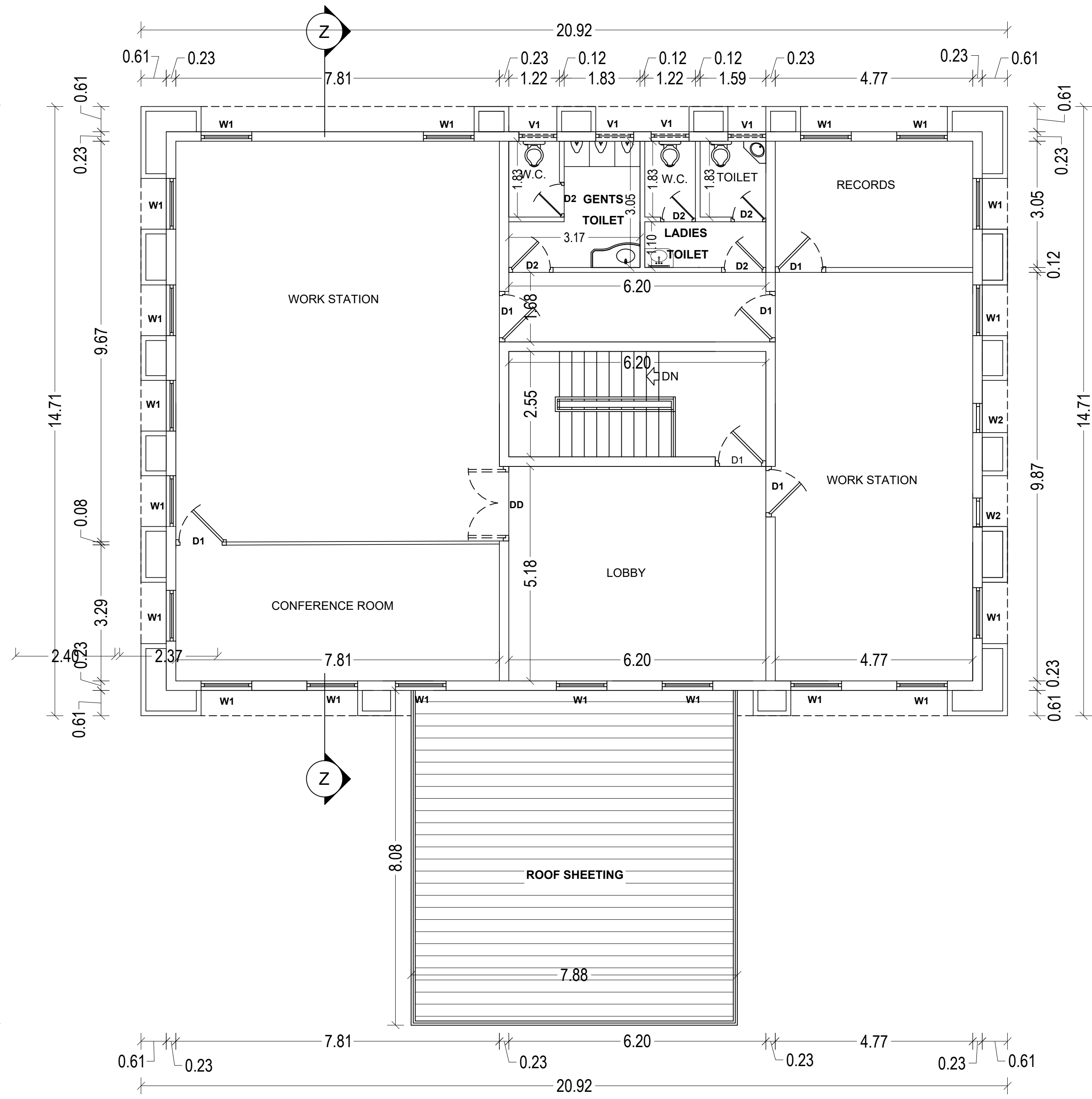
FIRST FLOOR PLAN ADMINISTRATIVE BLOCK
