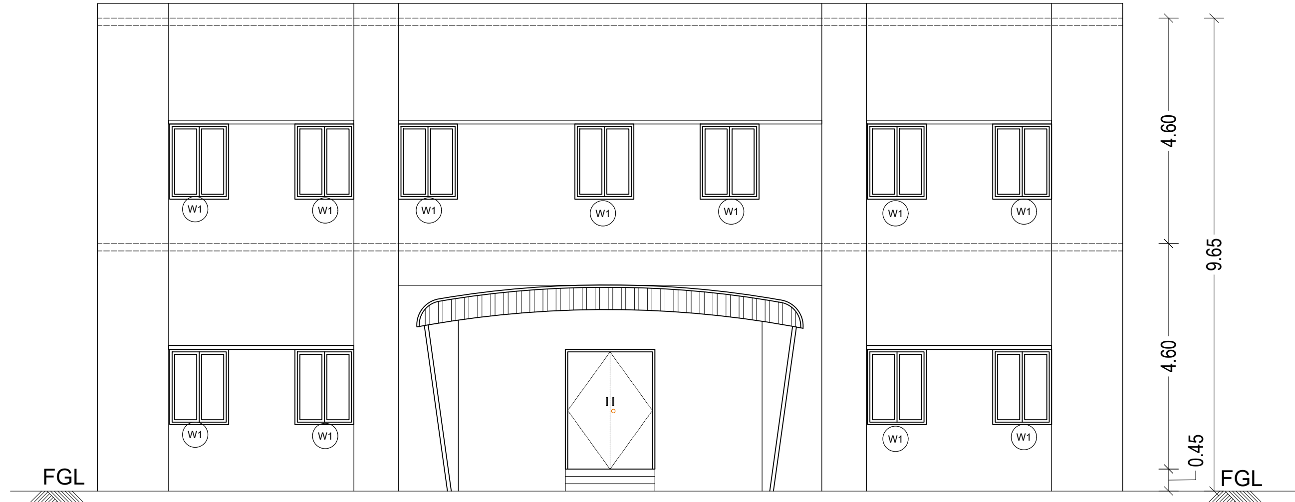
NORTH SIDE ELEVATION ADMINISTRATIVE BLOCK
