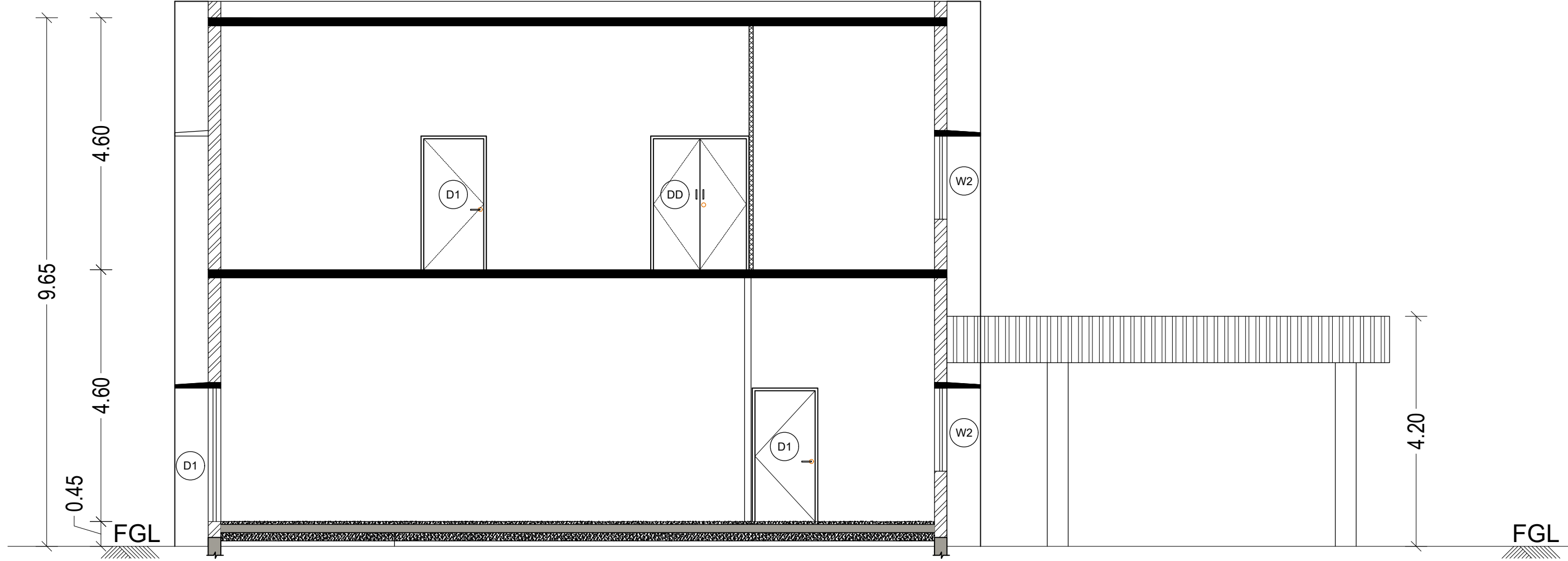
SECTION - ZZ ADMINISTRATIVE BLOCK
