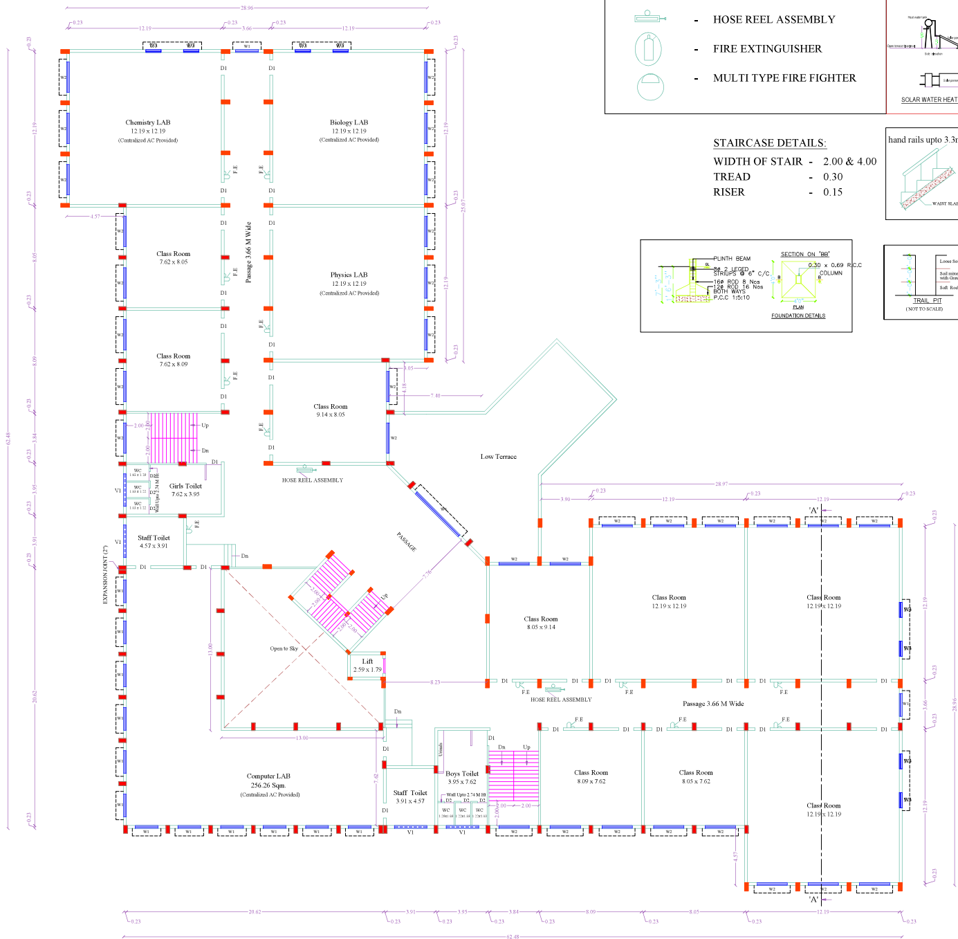
Proposed Third Floor Plan
