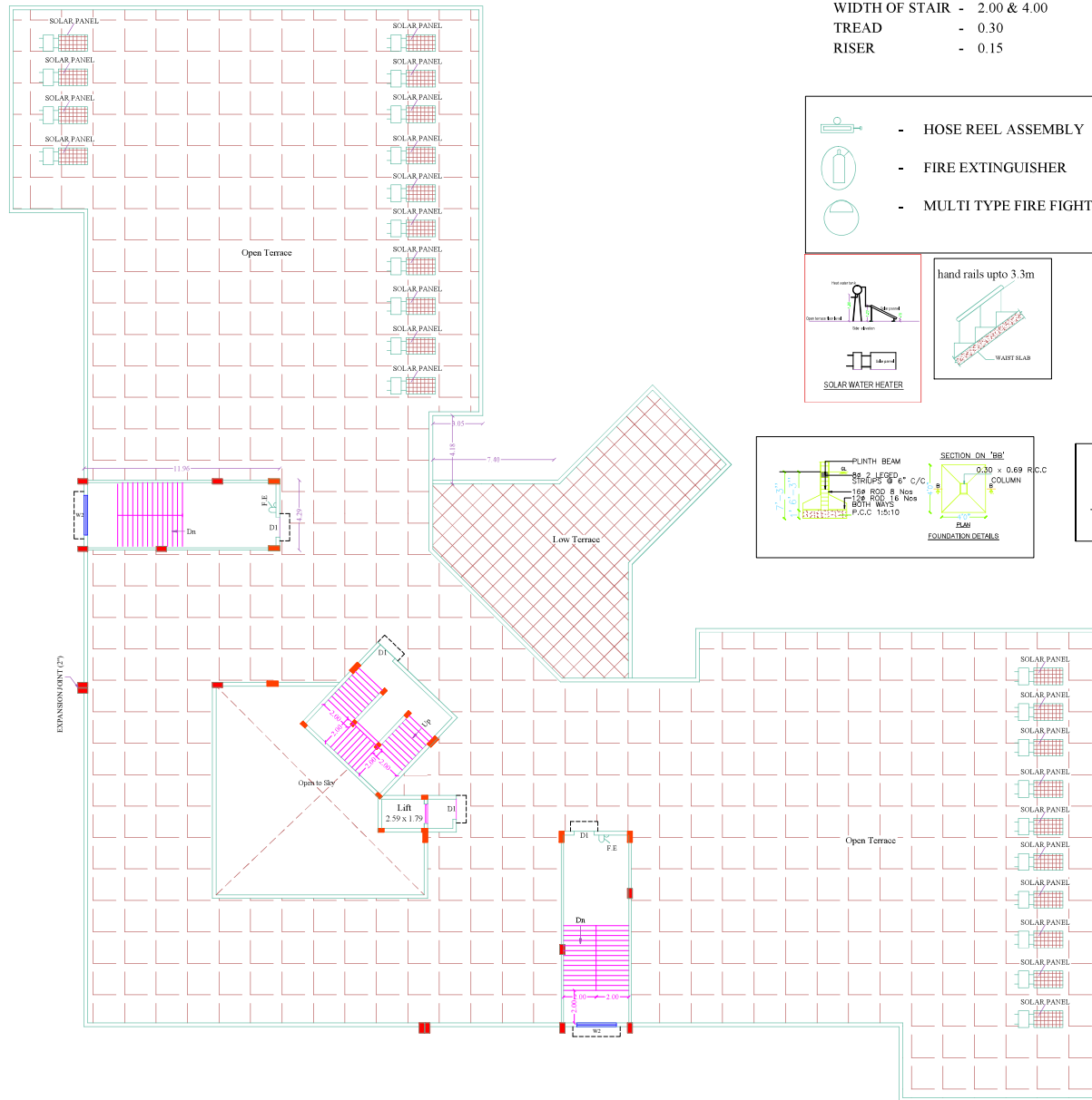
Existing Terrace Floor Plan
