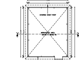
BLOCK-04_GROUND FLOOR PLAN
