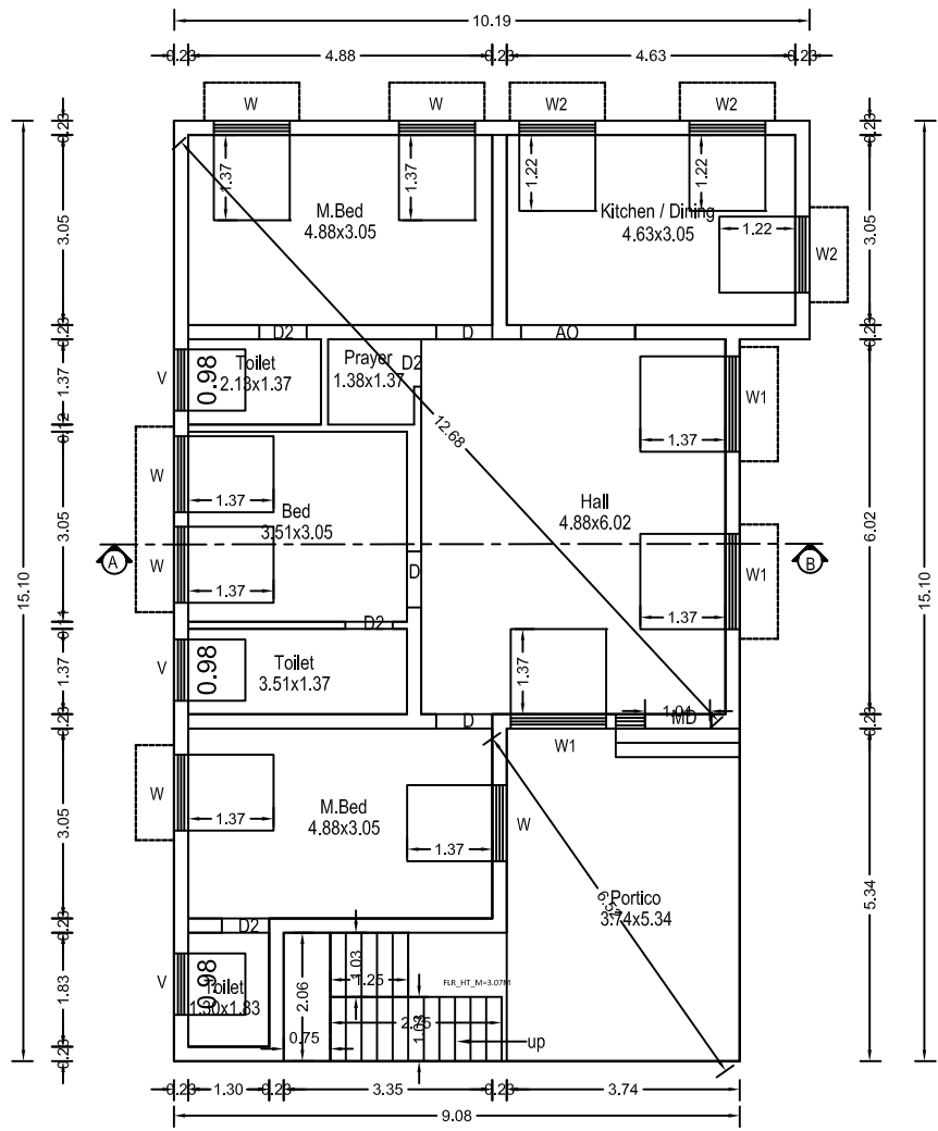
Plan Scale 1:100 Ground floor
