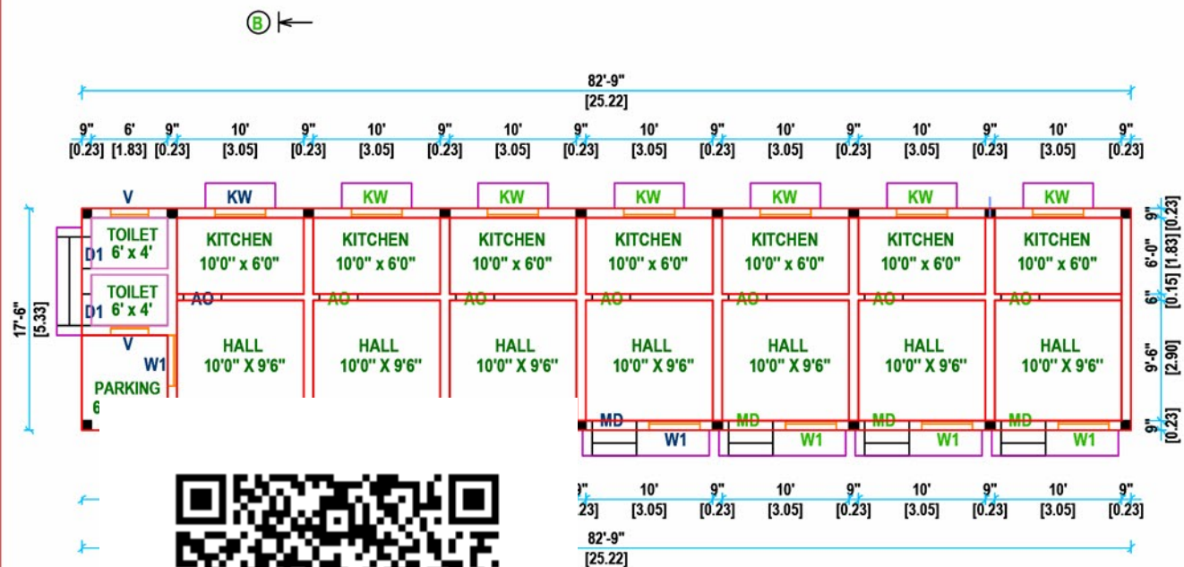
FLOOR PLAN
