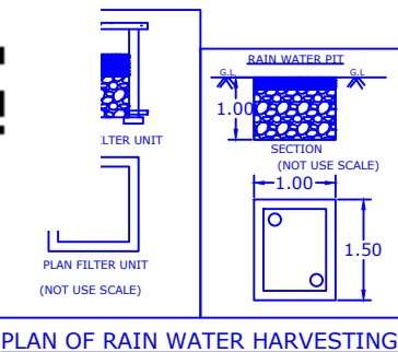
PLAN OF RAIN WATER HARVESTING
