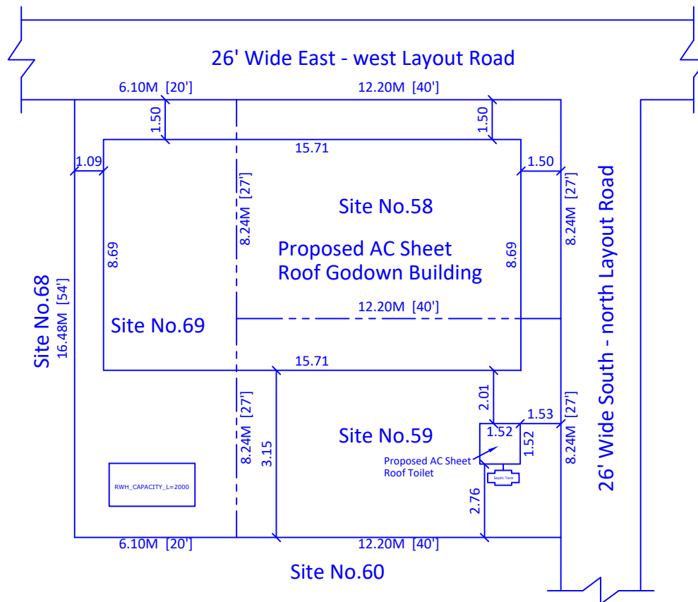
SITE PLAN
