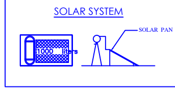
SOLAR SYSTEM
