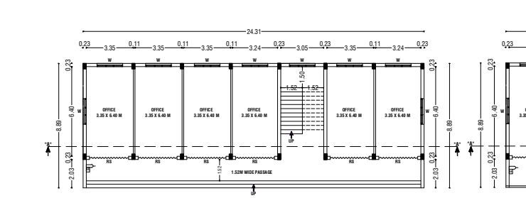
BLOCK-01-GROUND FLOOR PLAN
