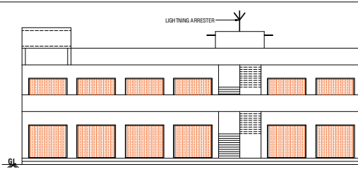
BLOCK-01 ELEVATION @ EAST SIDE
