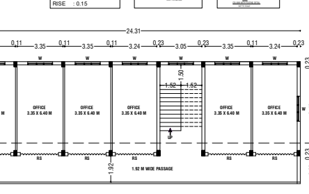
BLOCK-01-FIRST FLOOR PLAN
