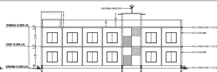
BLOCK-01 SECTION 'AA' @ WEST SIDE
