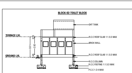
BLOCK-02-TOILET BLOCK
