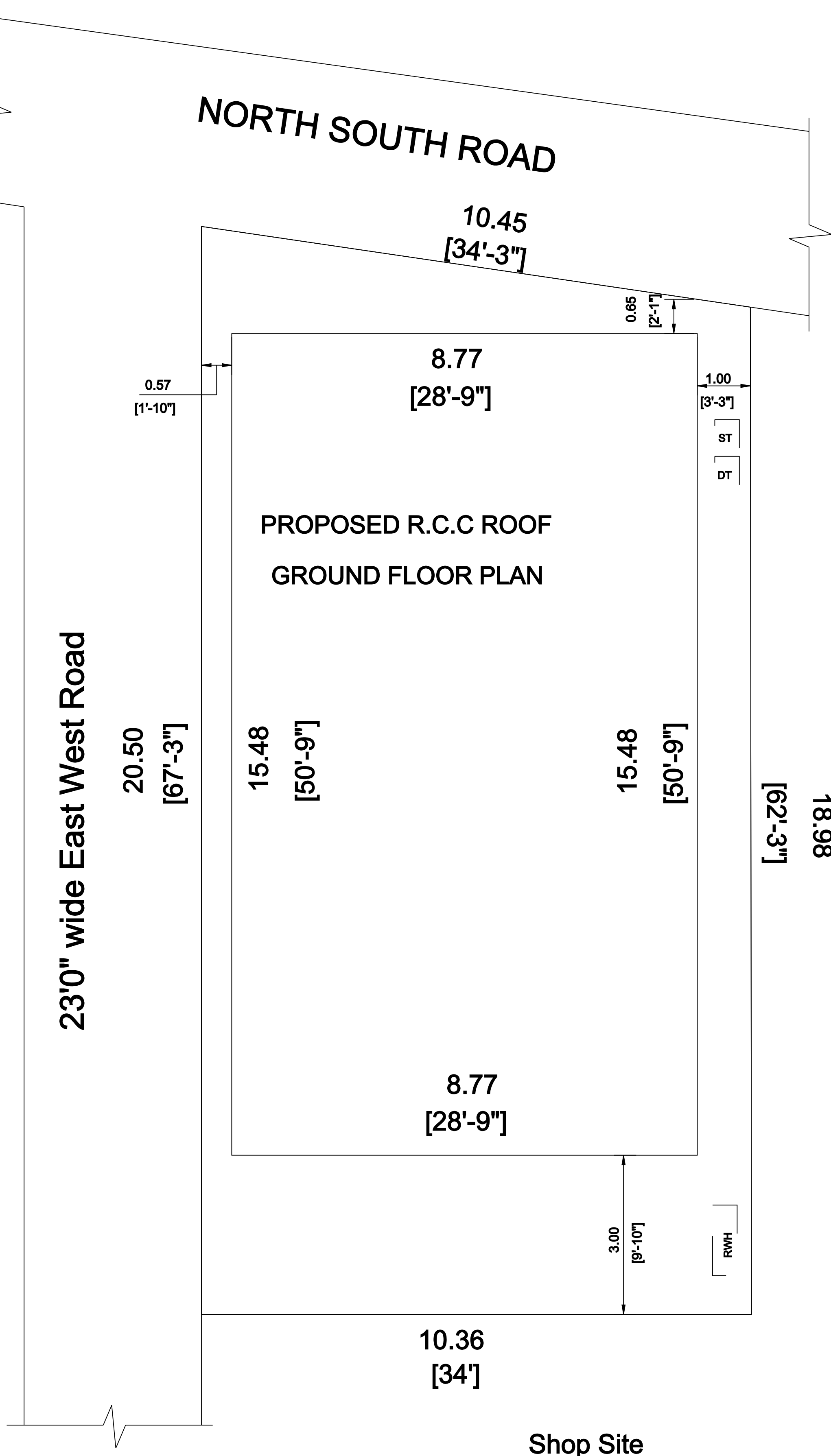
SITE PLAN
