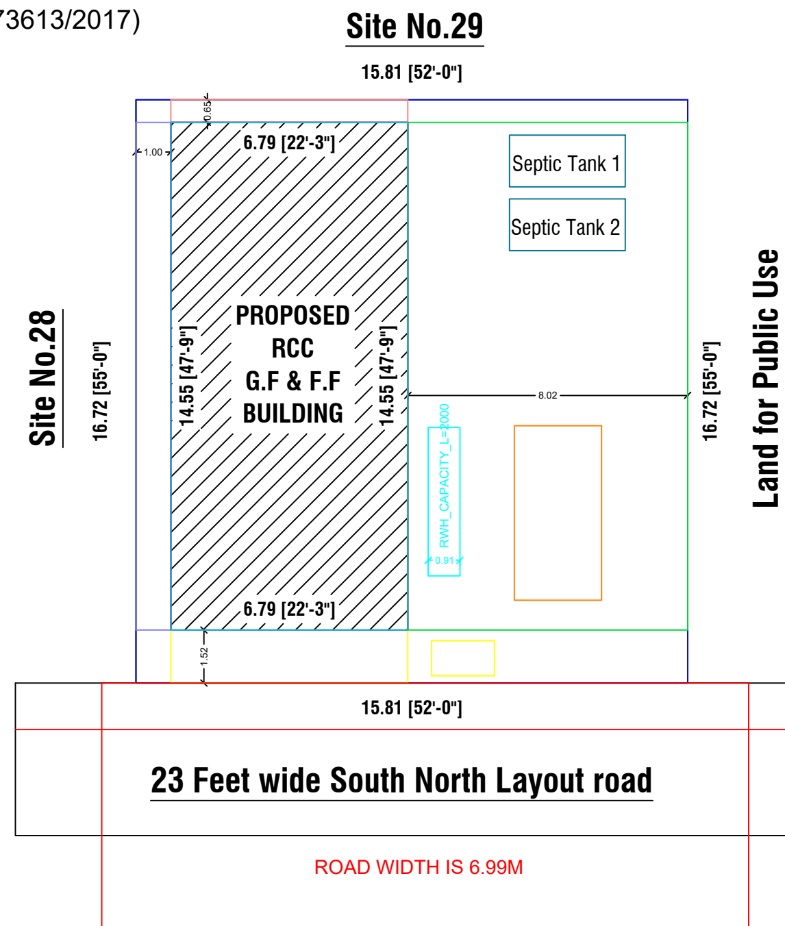
SITE PLAN
