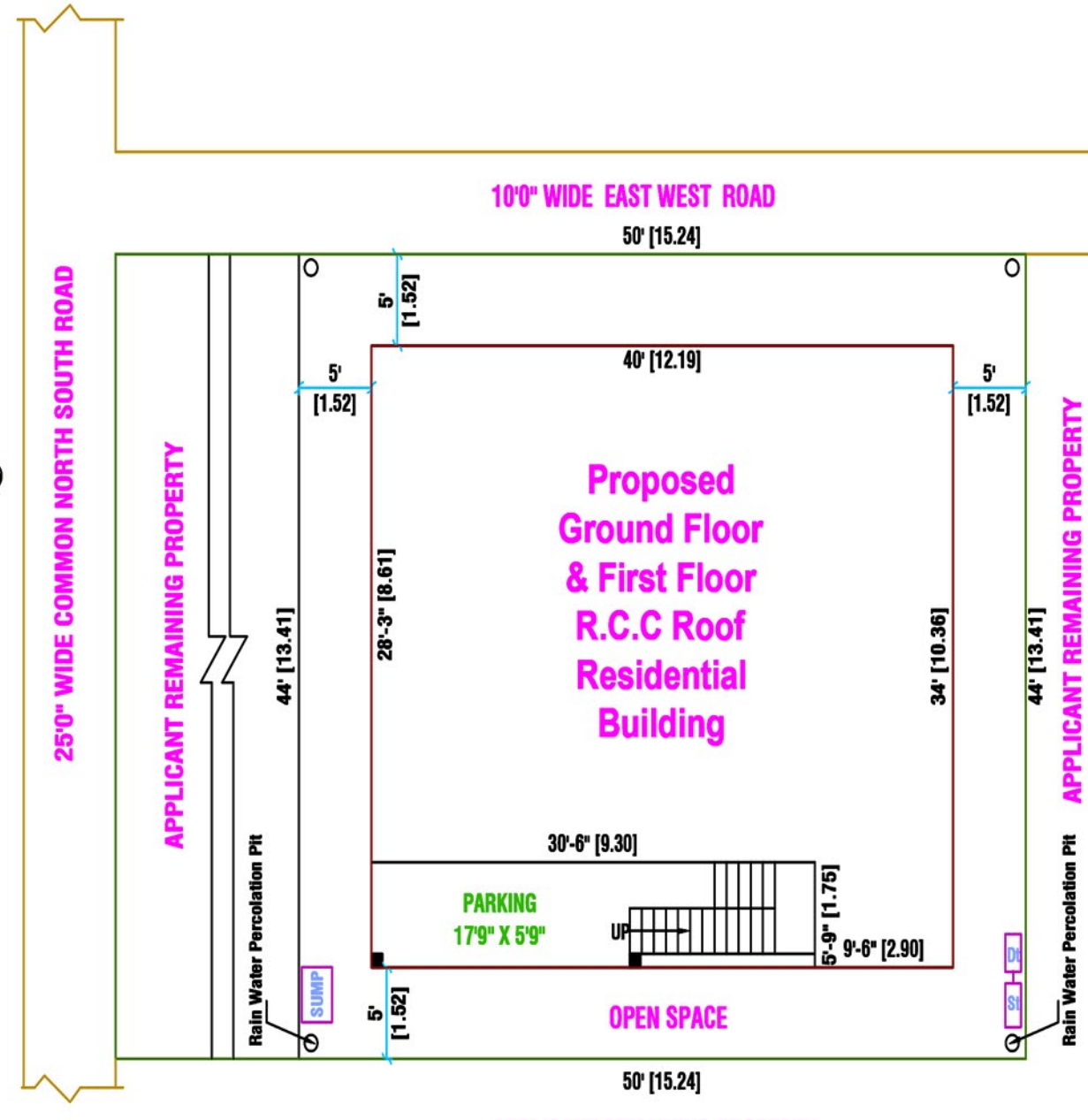
SITE PLAN SCALE 1" : 8' 0"
