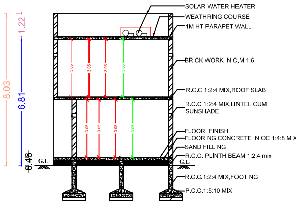
SECTION (B-B)
