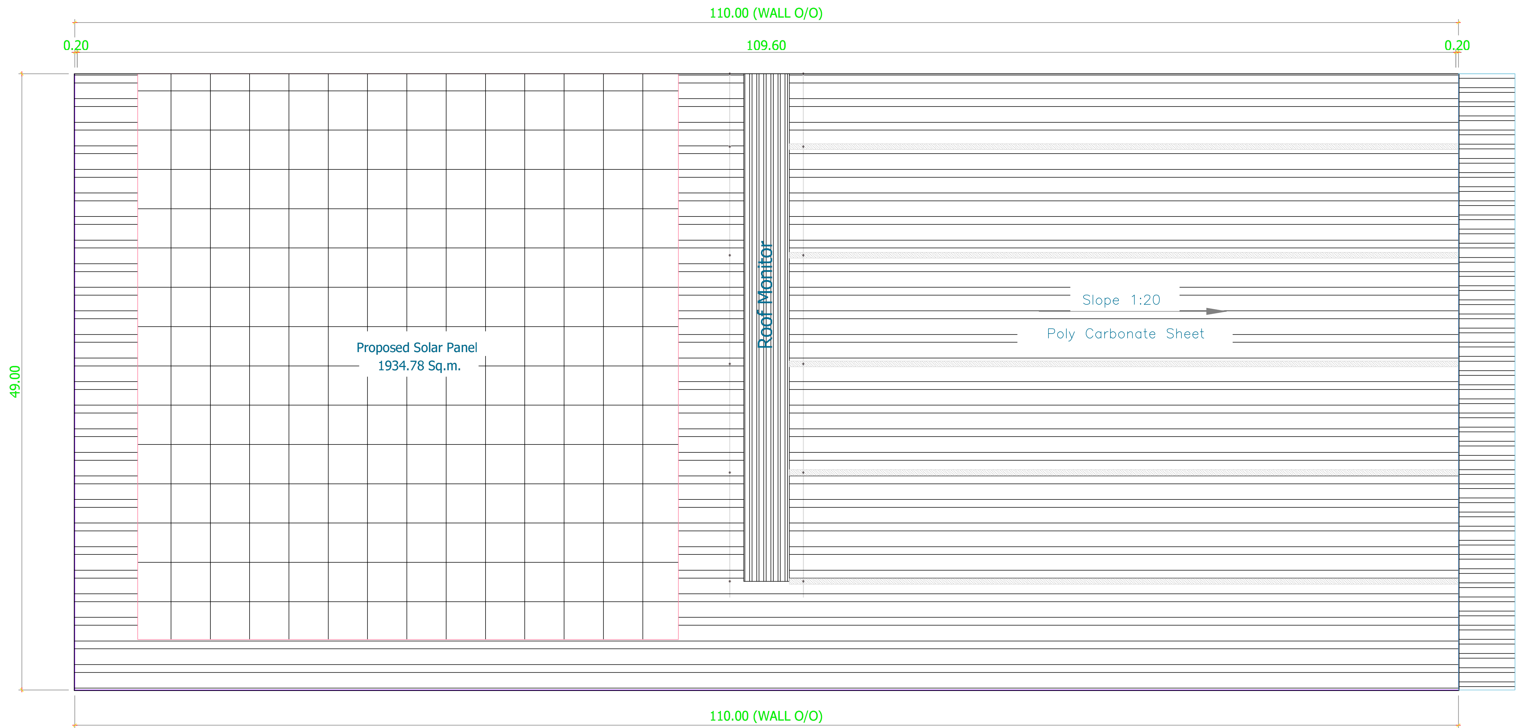
Roof Sheet Plan BLOCK A1
