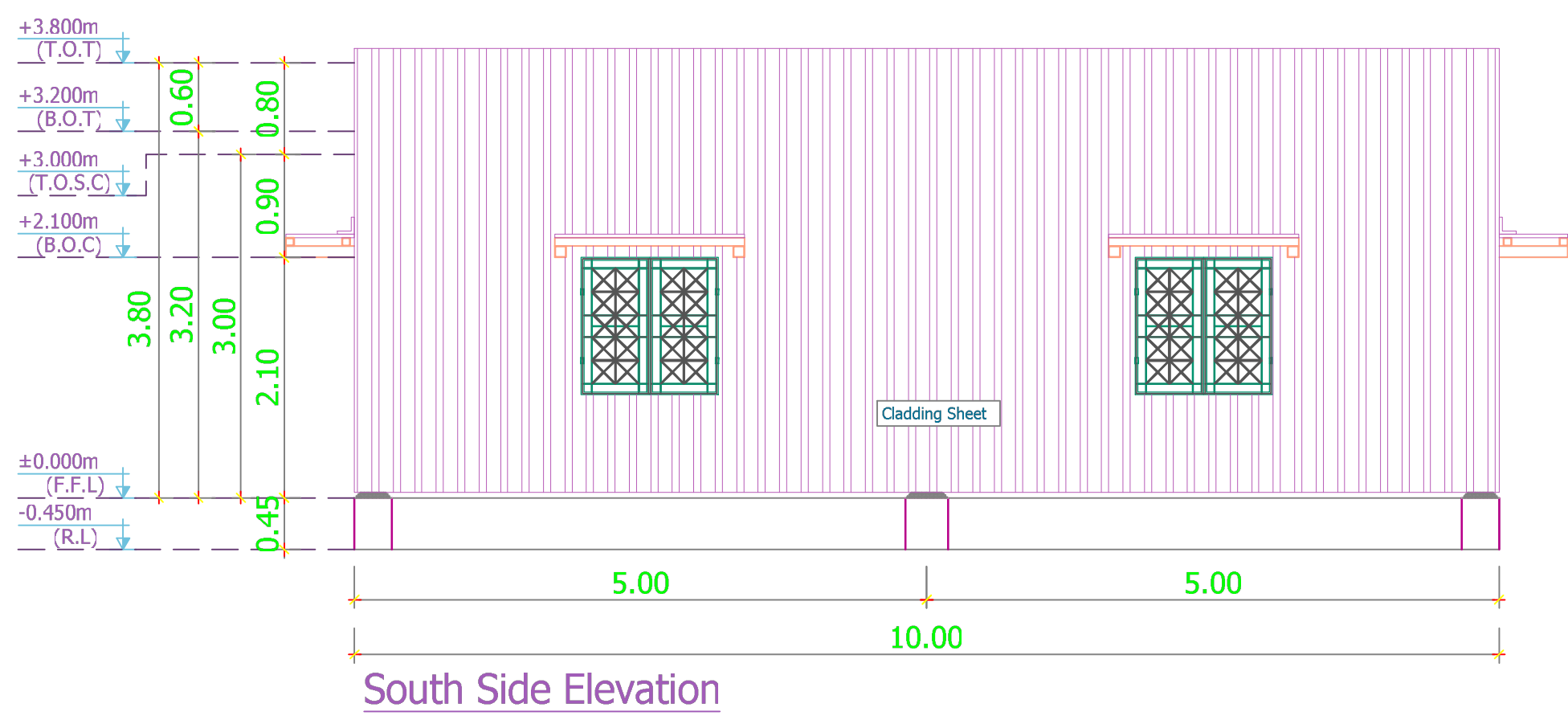
South Side Elevation
