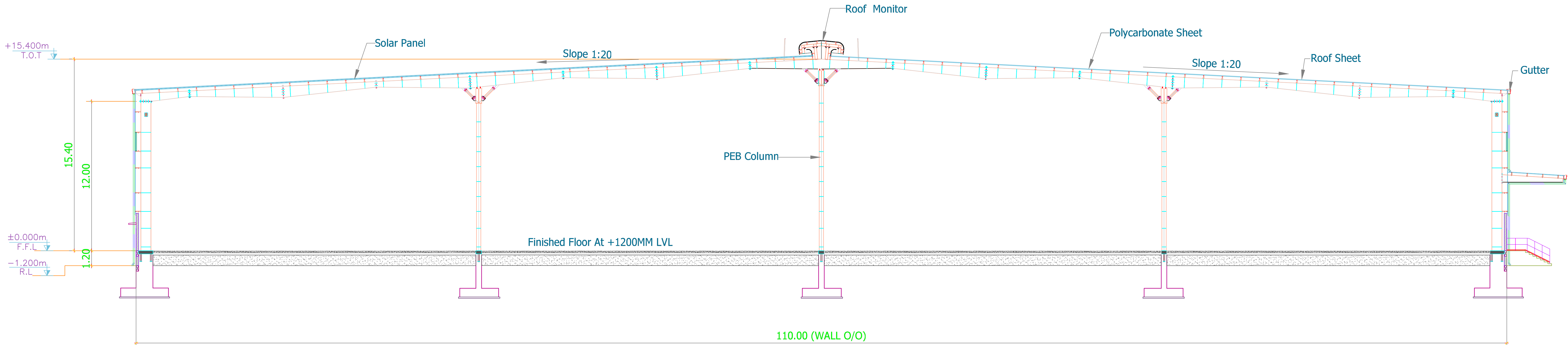
Section "D-D" BLOCK A1
