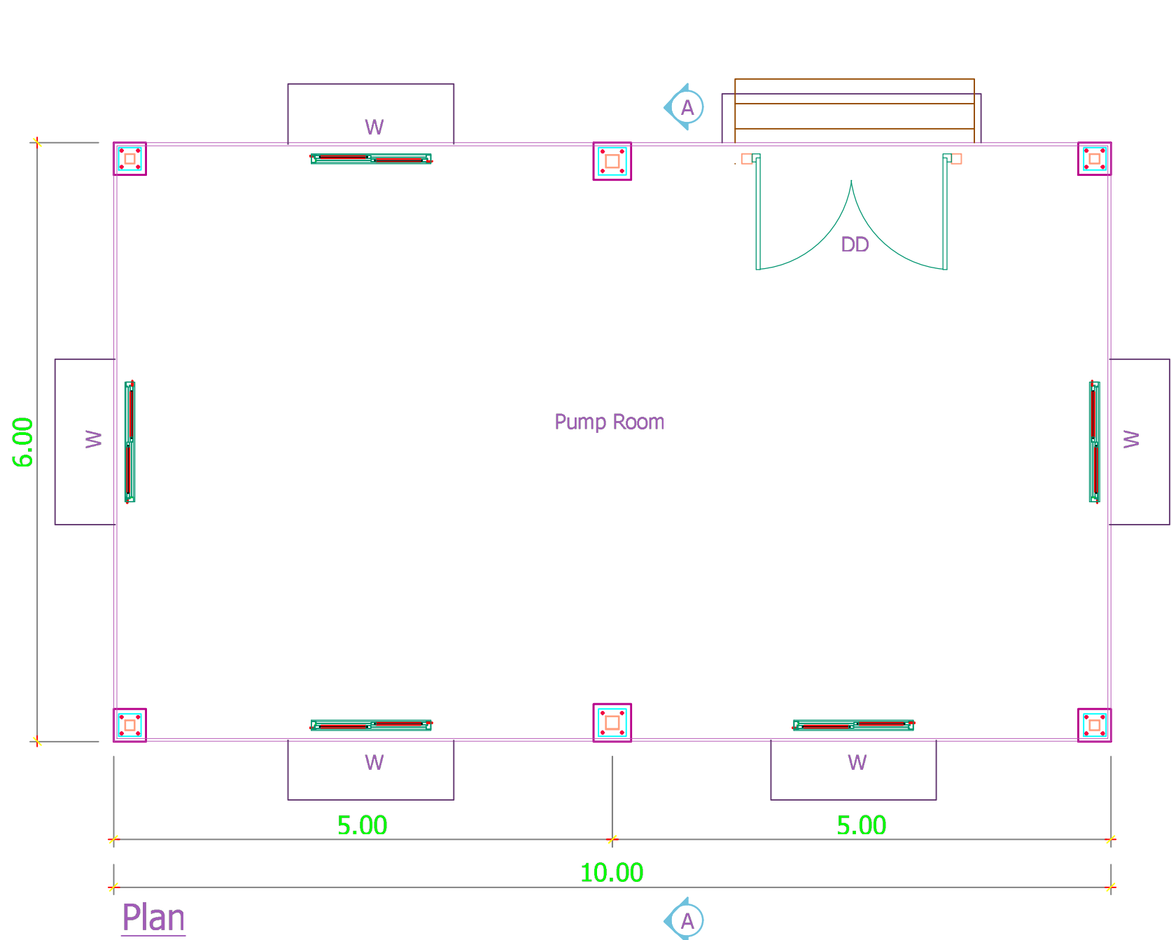
Plan
