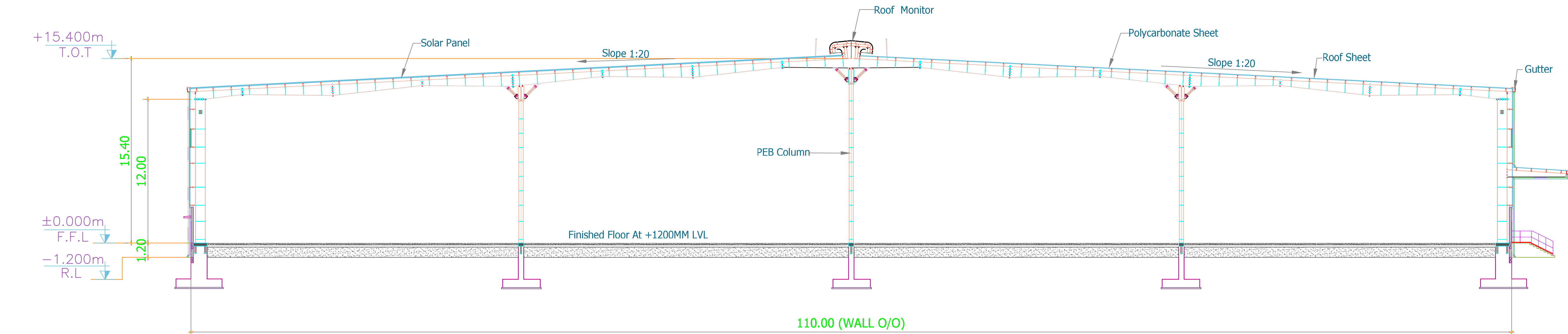
Section "C-C" BLOCK A3
